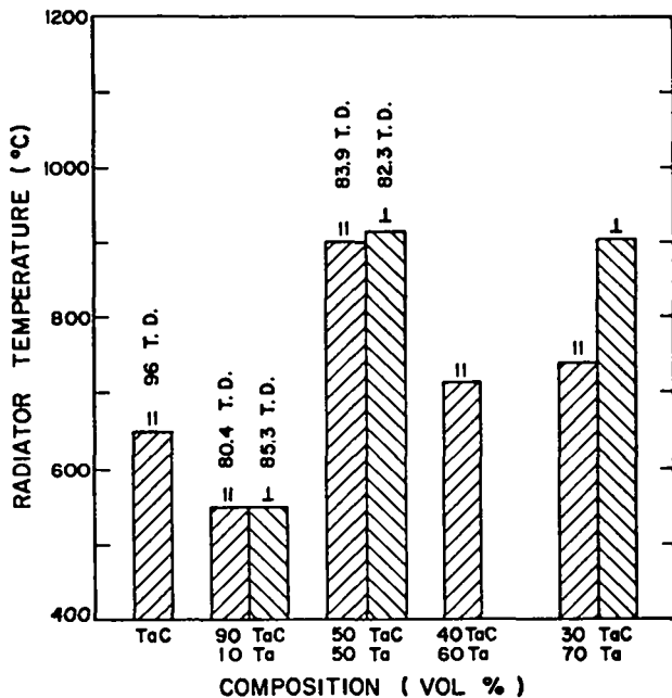
Fig. 1. Steady-state thermal-stress ranking of selected carbides.
