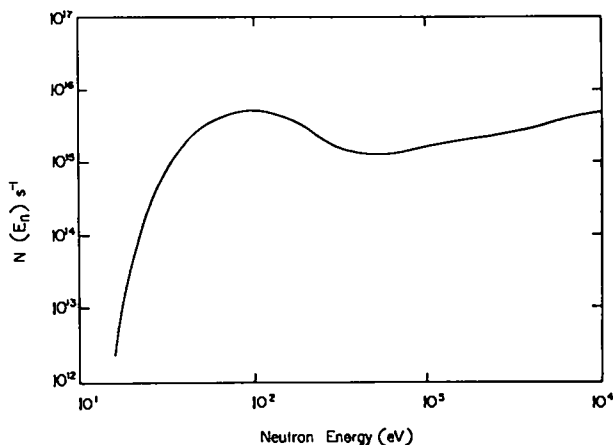
Fig. 2. The measured neutron beam flux incident on the 197 Au scattering foils shown as a function of energy.
