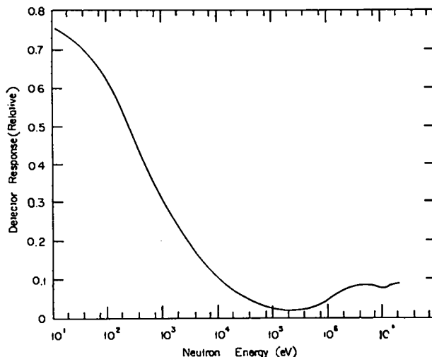
Fig. 3. Response of the high-pressure 3 He neutron detectors as a function of incident neutron energy.
