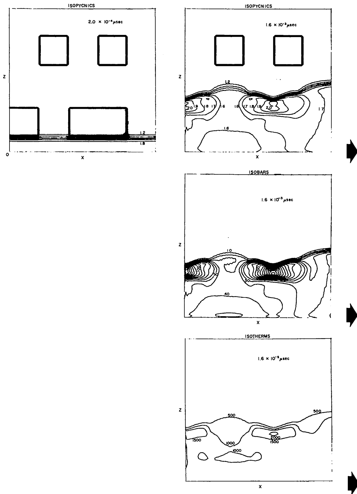
Fig. 11. The interaction of an 85-kbar shock in a 1.6 \times 10^{-3} -cm half-width, 1.6 \times 10^{-3} -cm-high slab of nitromethane with four rectangular holes. Chemical reaction is not permitted. The interval between isopycnics is 0.1 cm/cc, that between isobars is 10 kbar, and that between isotherms is 500° Kelvin. The isopycnics show the hole geometry.
