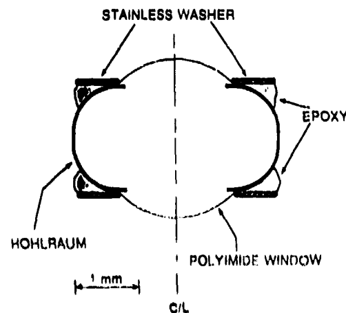
Figure 1. A high pressure gas-filled hohlraum.
