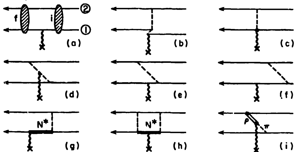
FIG. 2. Time-ordered Feynman diagrams which contribute to exchange currents.
