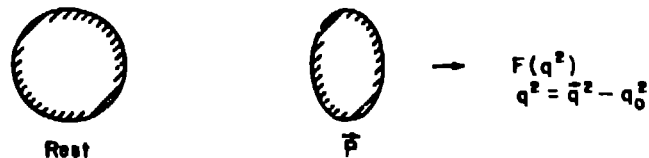
FIG. 6. Schematic Lorentz contraction effect on a nucleus.
