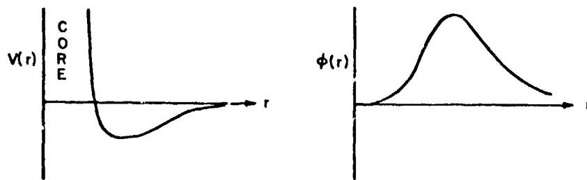
FIG. 5. Schematic depiction of two-nucleon potential, V , and deuteron wave function, \phi .
