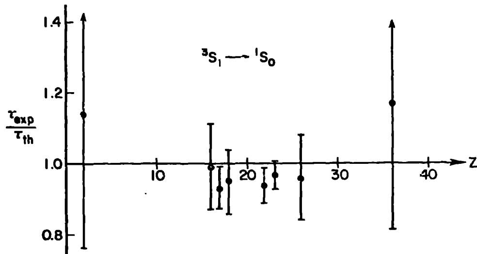
FIG. 8. Experimental to theoretical lifetime ratio appropriate to the ^3S_1 to ^1S_0 transition in Helium-like ions.
