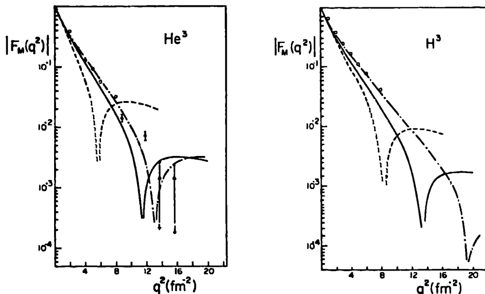
FIG. 3. {}^3\text{He} and {}^3\text{H} magnetic form factors vs. momentum transfer.
