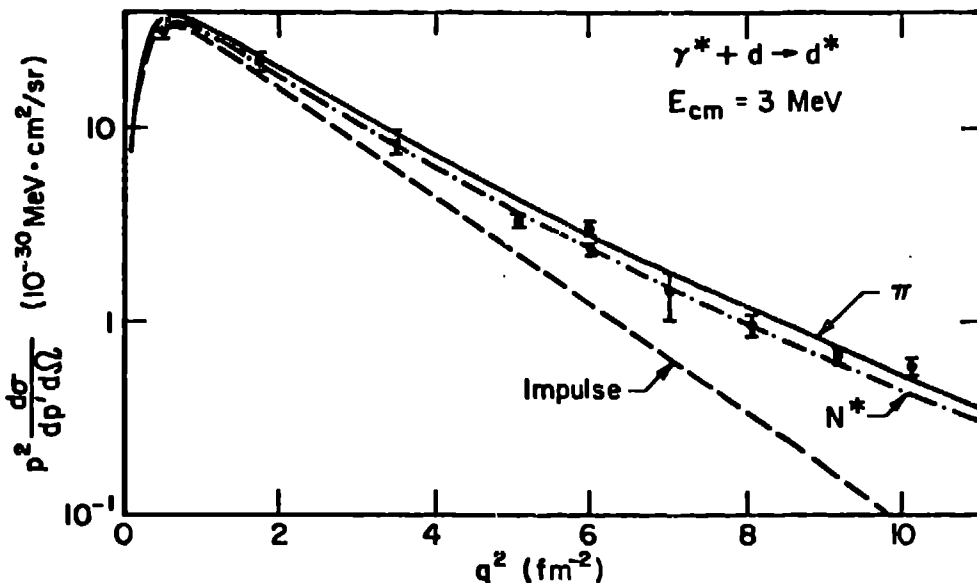
FIG. 4. Electro-excitation cross section for d \rightarrow d^*(^1S_0) vs. momentum transfer.
