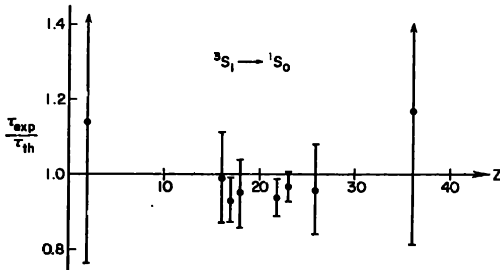
FIG. 8. Experimental to theoretical lifetime ratio appropriate to the ^3S_1 to ^1S_0 transition in Helium-like ions.
