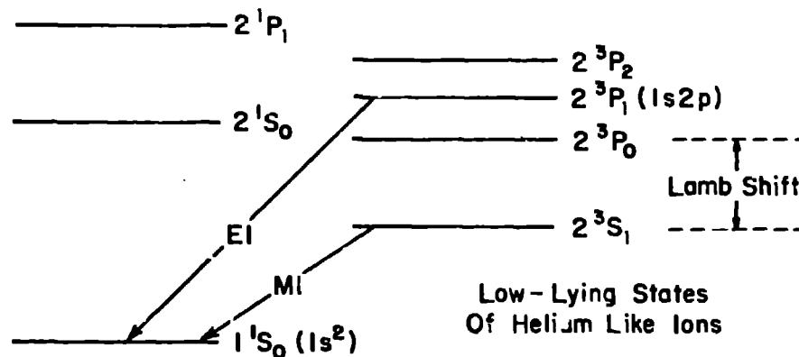
FIG. 7. Low-lying states of Helium-like ions.
