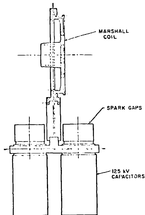
Fig. 5. Marshall coil test stand.
