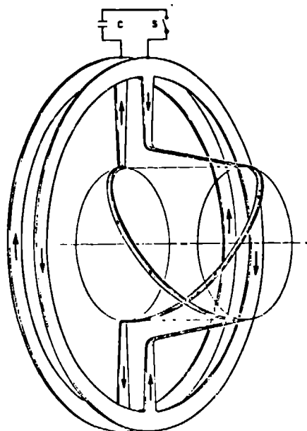
Fig. 1. Simple (two-conductor) Marshall coil showing current flow.
