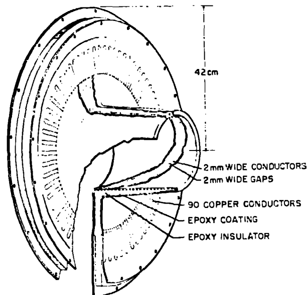
Fig. 4 Cutaway of the Prototype Marshall implosion coil.
