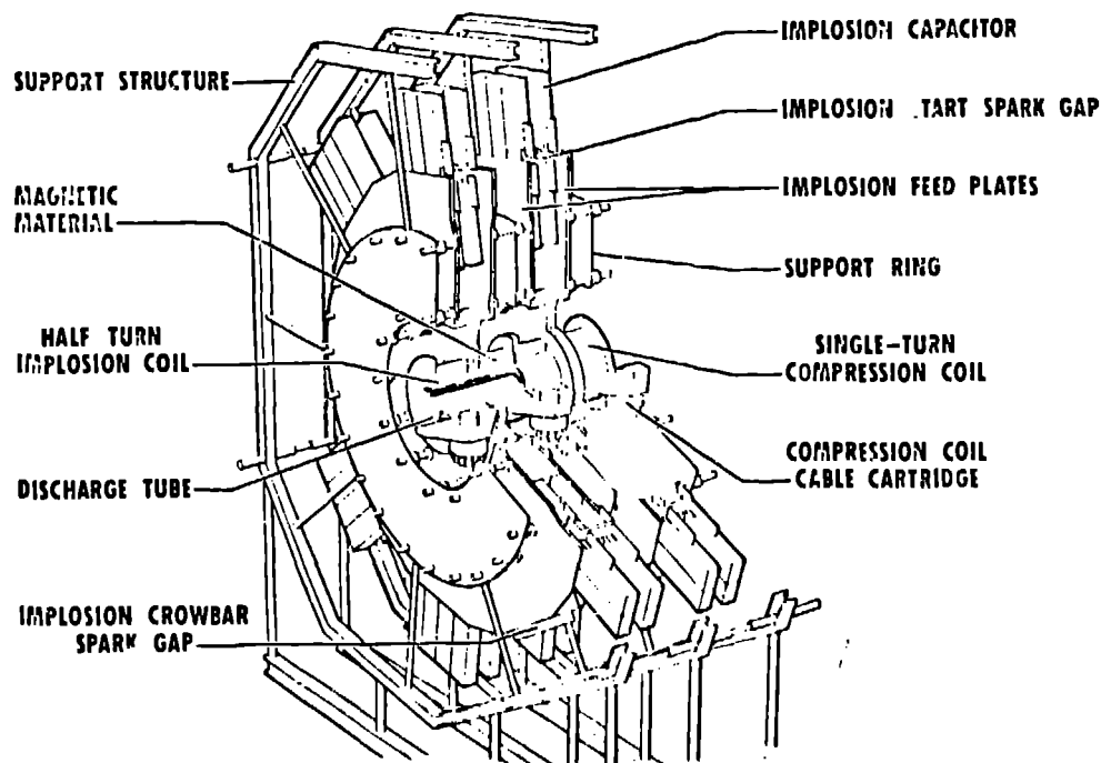
Fig. 3. Staged Theta Pinch modular assembly using Marshall implosion coils and a radial implosion power supply.
