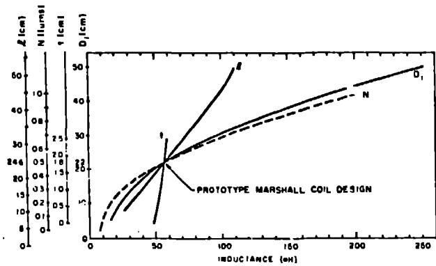
Fig. 2. Calculated Marshall coil inductance by variation of individual parameters.
