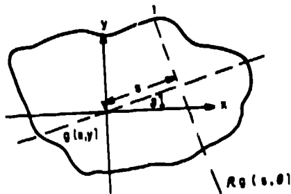
Figure 1: Each projection is an estimate of the line integral of the function g(x,y) , where the line of integration is specified by the parameters s and \theta . Geometrical relation between a two-dimensional source g(x,y) and the measured projection Rg(s,\theta) .
