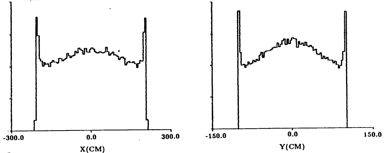
Beam Profiles at APT Target
