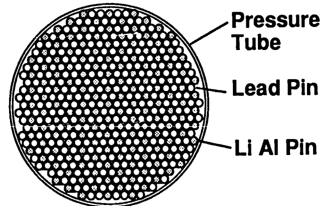
CROSS SECTION OF PRESSURE TUBE
