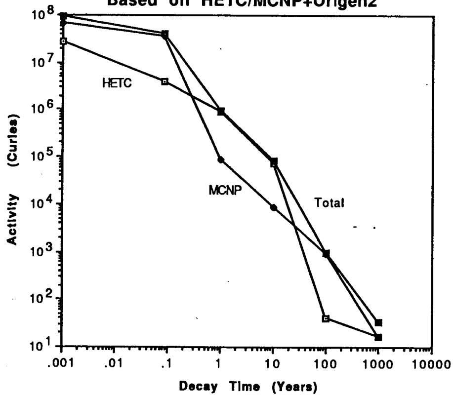
Total Radioactivity from Target Components Based on HETC/MCNP+Origen2
