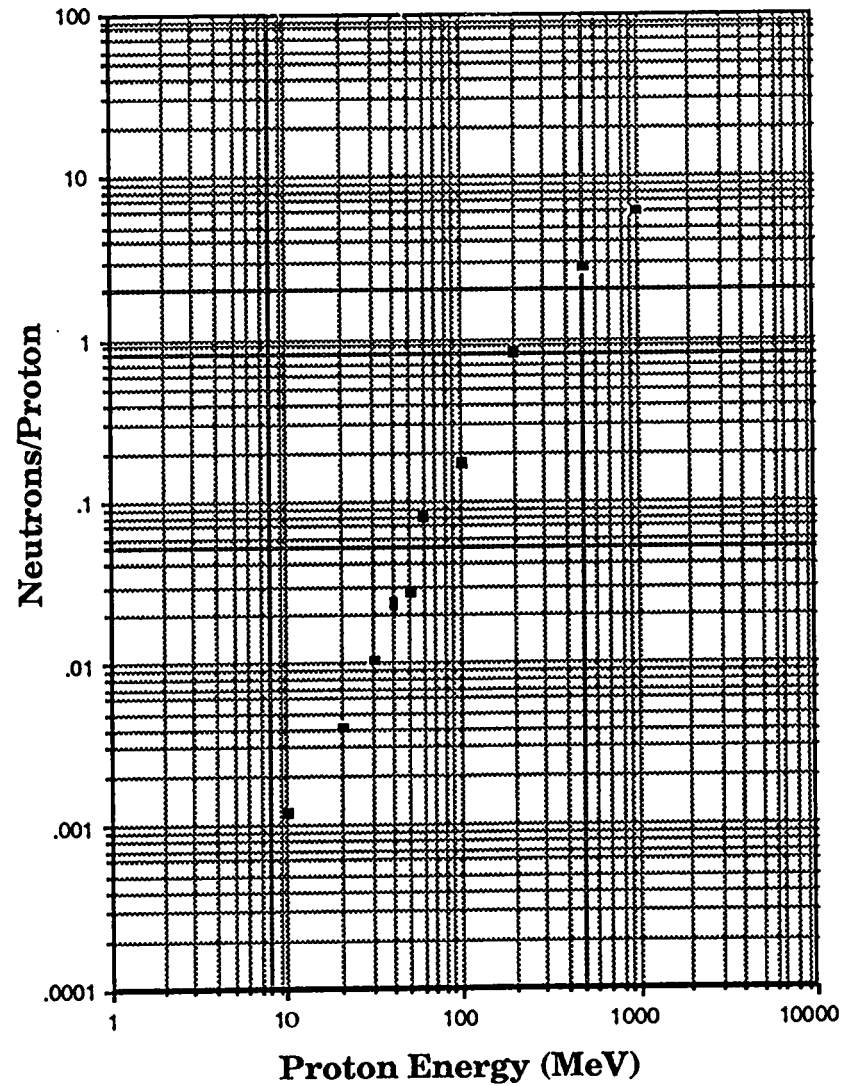
Neutron Yield vs E_p for Copper/Iron
