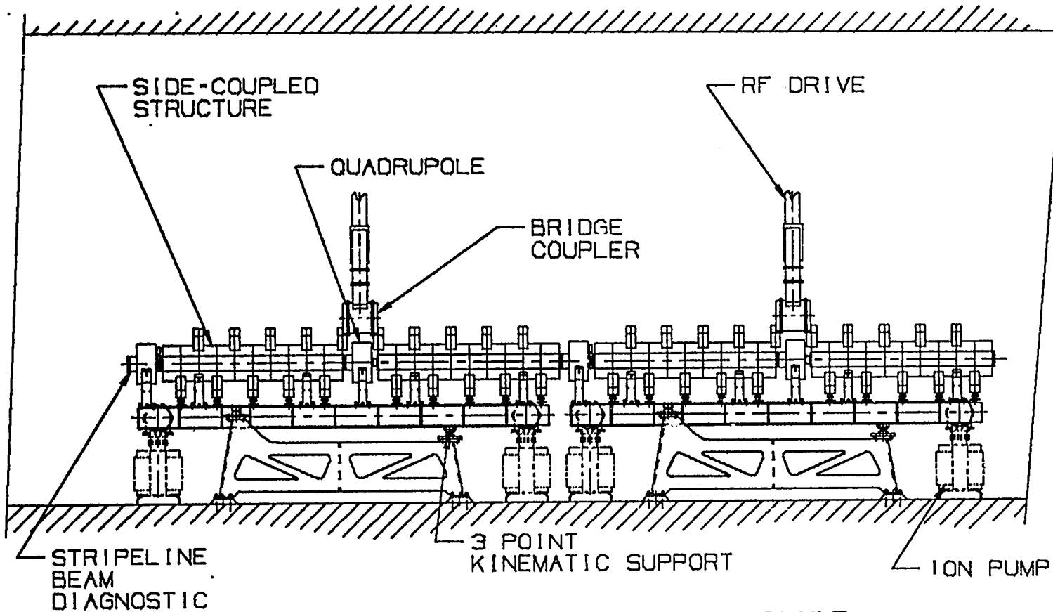
APT 10-CELL CCL ACCELERATING MODULE
