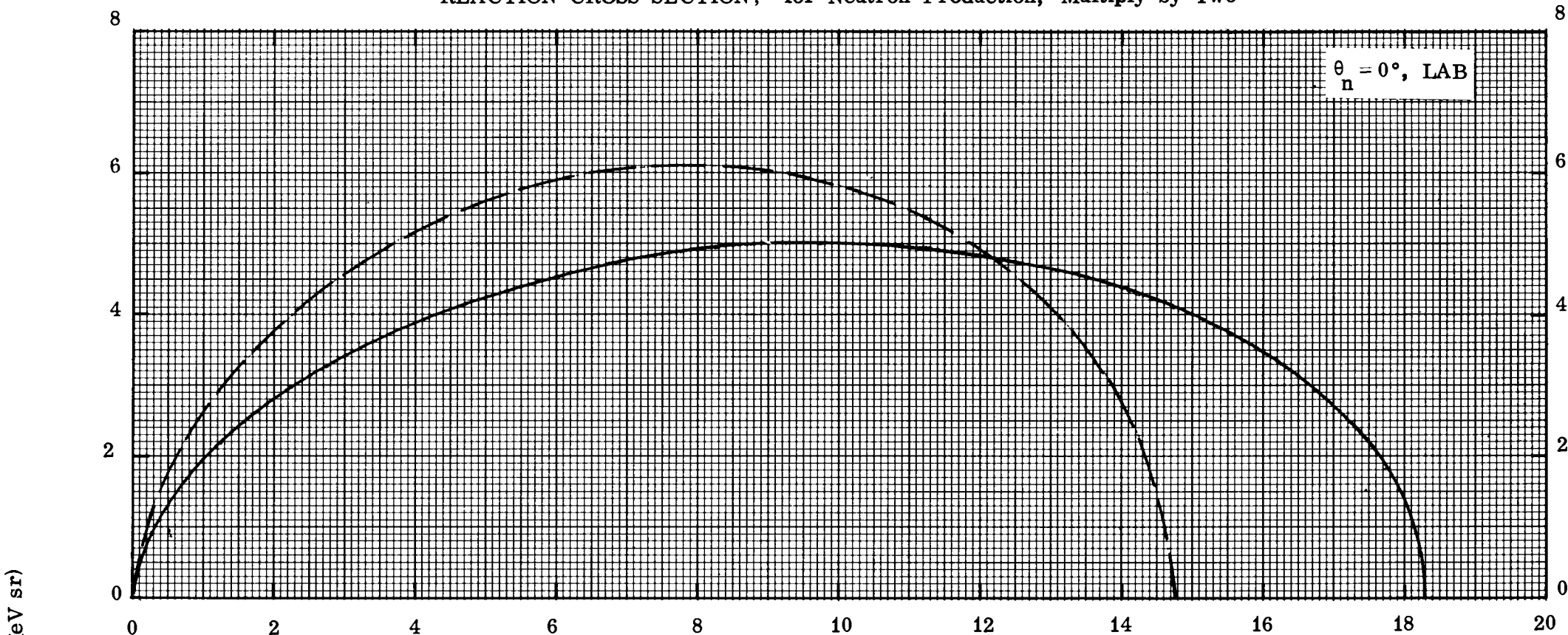
REACTION CROSS SECTION; for Neutron Production, Multiply by Two
