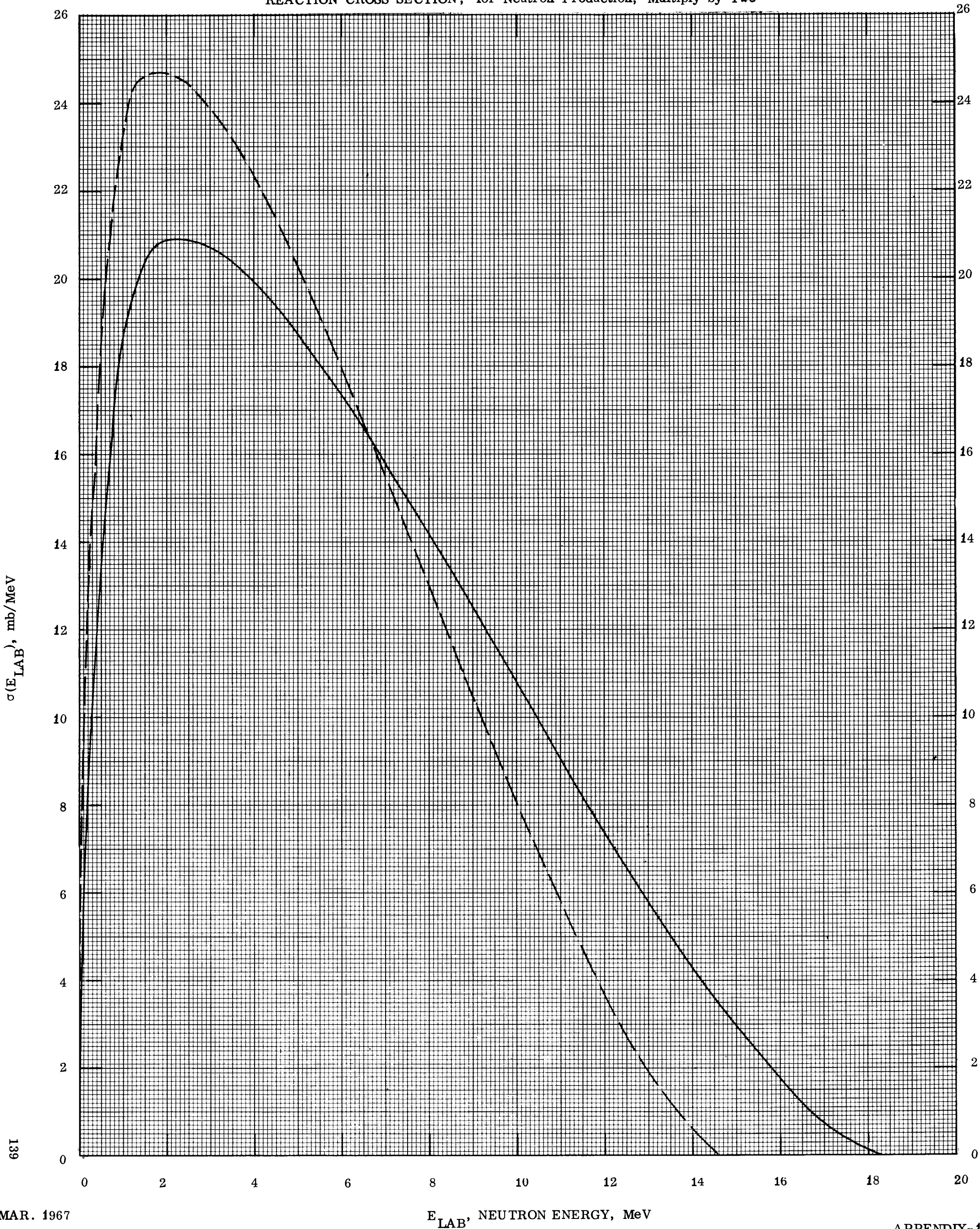
REACTION CROSS SECTION; for Neutron Production, Multiply by Two
