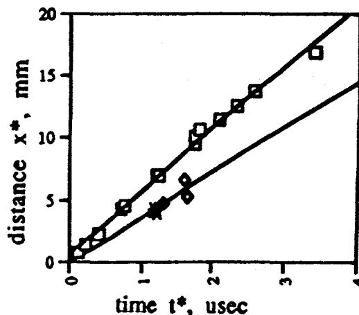
Figure 5. The run distance for the heated PBX-9502 sample ( \blacksquare ) is comparable to the run distance for PBX-9502 at initial density of 1.825 ( \blacklozenge ), but differs from the run for cold PBX-9502 ( \square )
