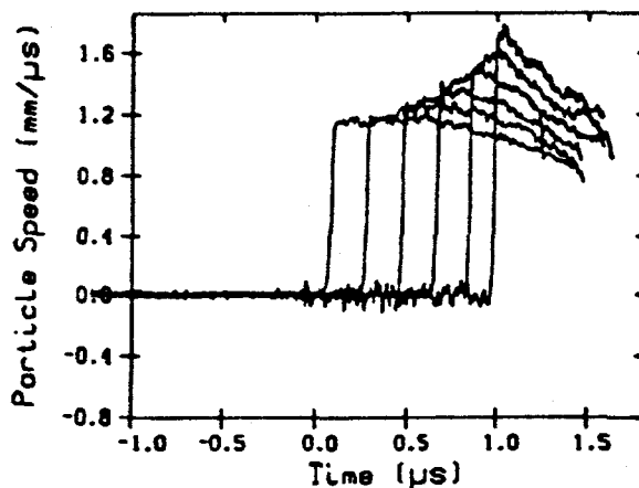
Figure 4. Detonation behavior of PBX-9502 at 100°C.
