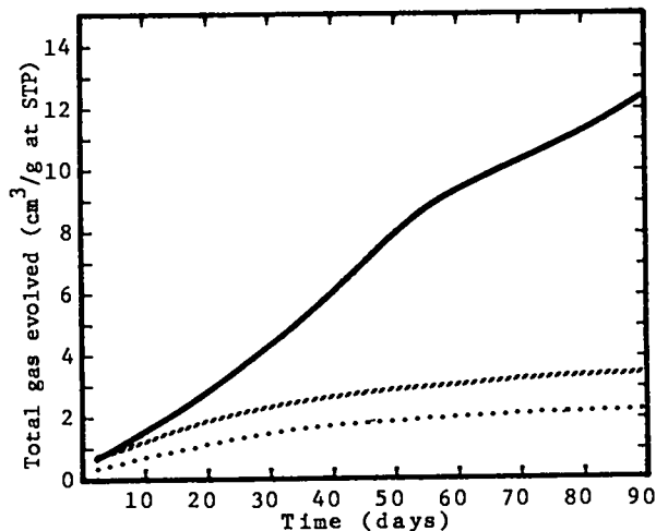
Fig. 8. DPPM (Dipicrylpyromellitide)
