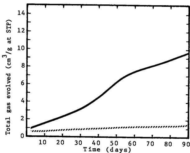
Fig. 6. DODECA (Dodecanitroquaterphenyl)
