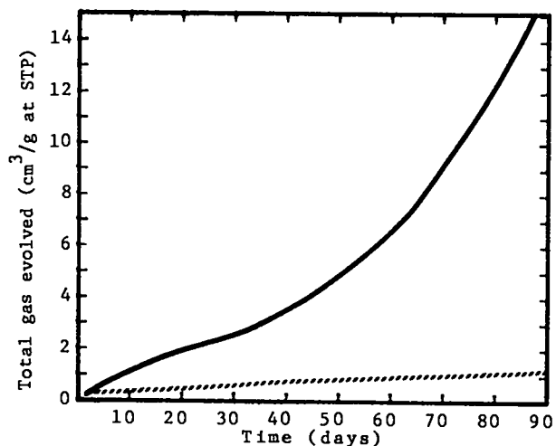
Fig. 2. BTX (Dinitropicrylbenzotriazole)
