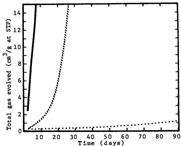
Fig. 12. HNDS (Hexanitrodiphenylsulfone)
