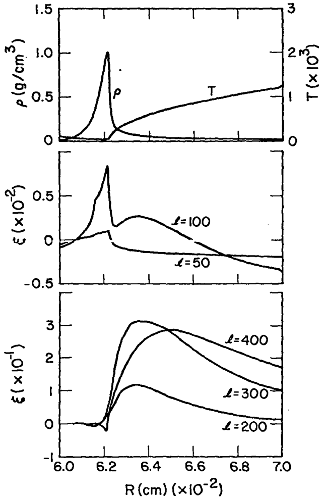
Fig. 3(a). Zeroth order density and temperature for an A=20 shell. (b) \xi_r (radial displacement) for various \ell -mode values. (c) Same as (b).
