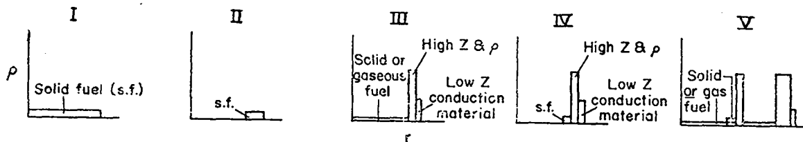
Fig. 1. Five types of laser fusion pellets.
