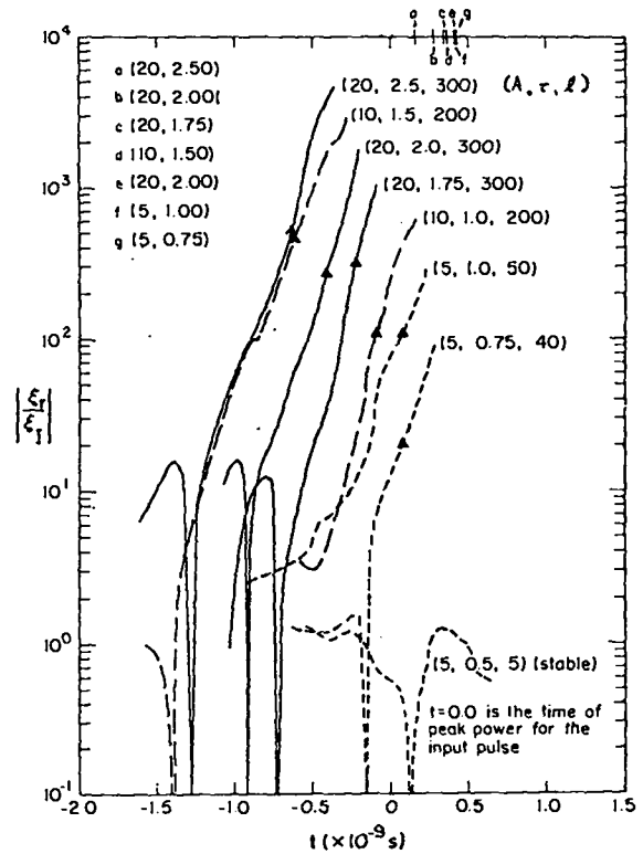
Fig. 4. Values of \xi_r measured at the ablation surface for the \ell -mode of maximum growth for fixed A and \tau .
