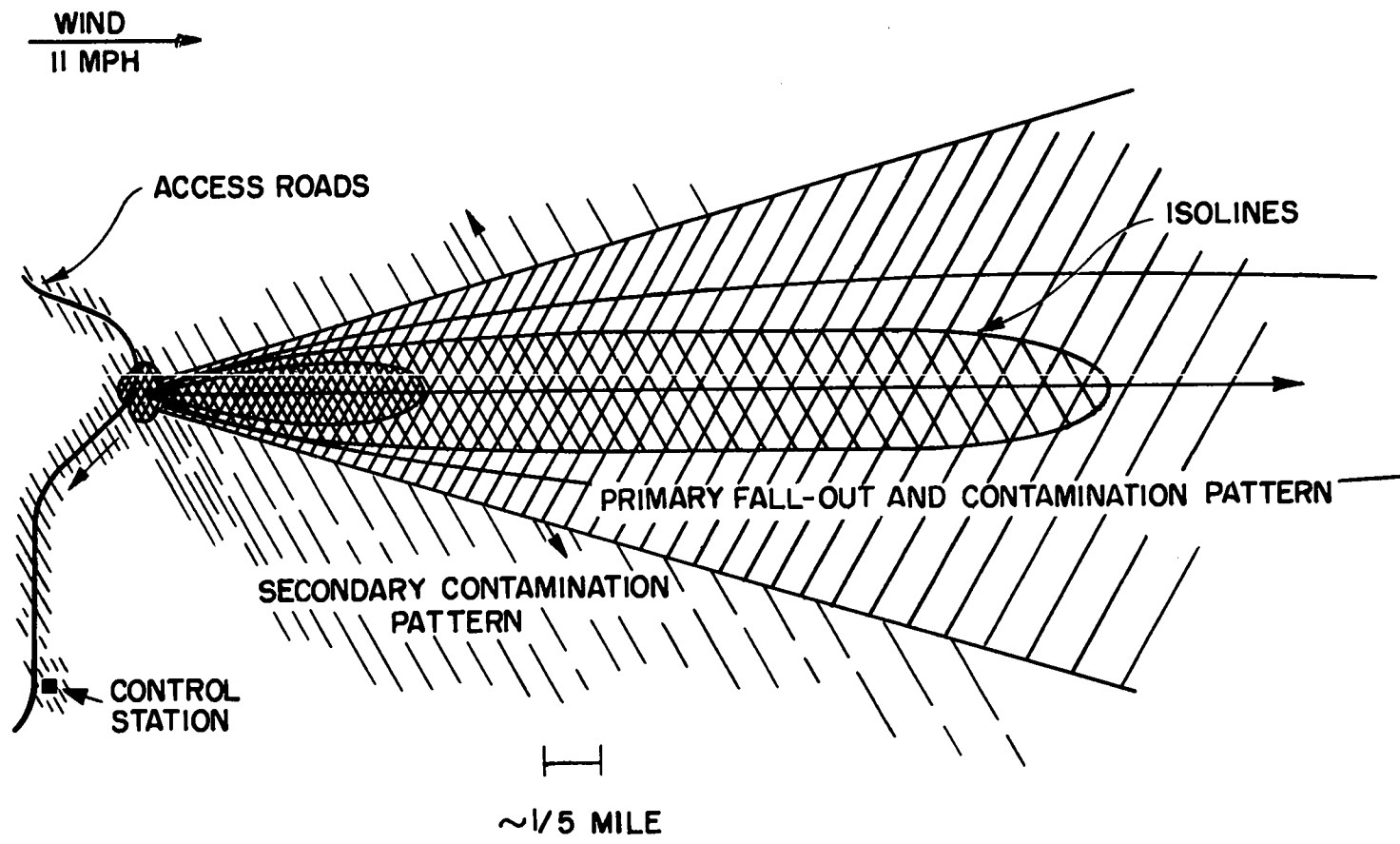
Fig. 1 Idealized fall-out and ground contamination pattern as might be expected from Sutton's formula, assuming release at ground level and wind speed of 11 mph
