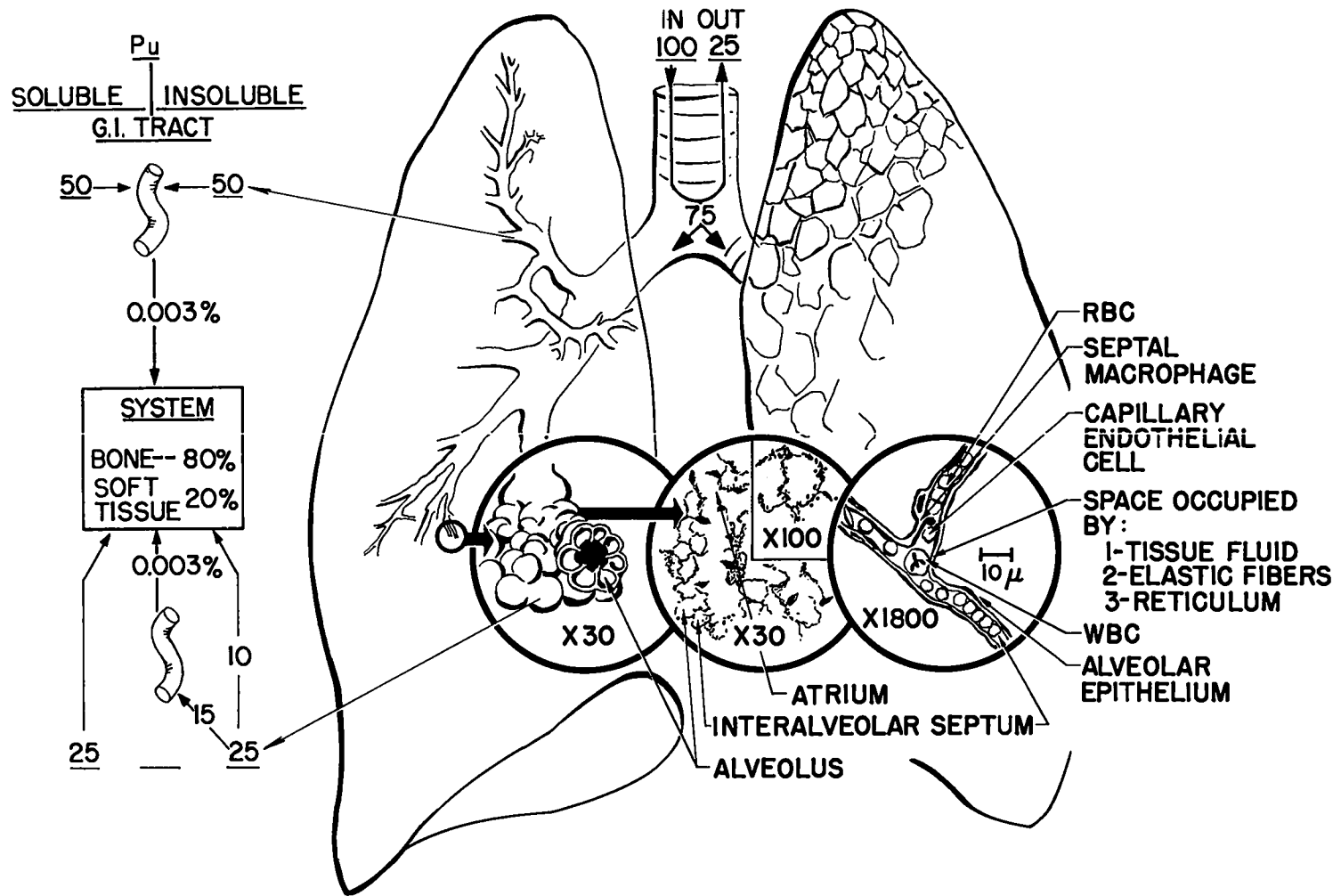
Fig. 2 General model for the fate of radioactive particles (0.5-10 μ) in the lung (Tripartite Conference, Harriman, N. Y., 1954)
