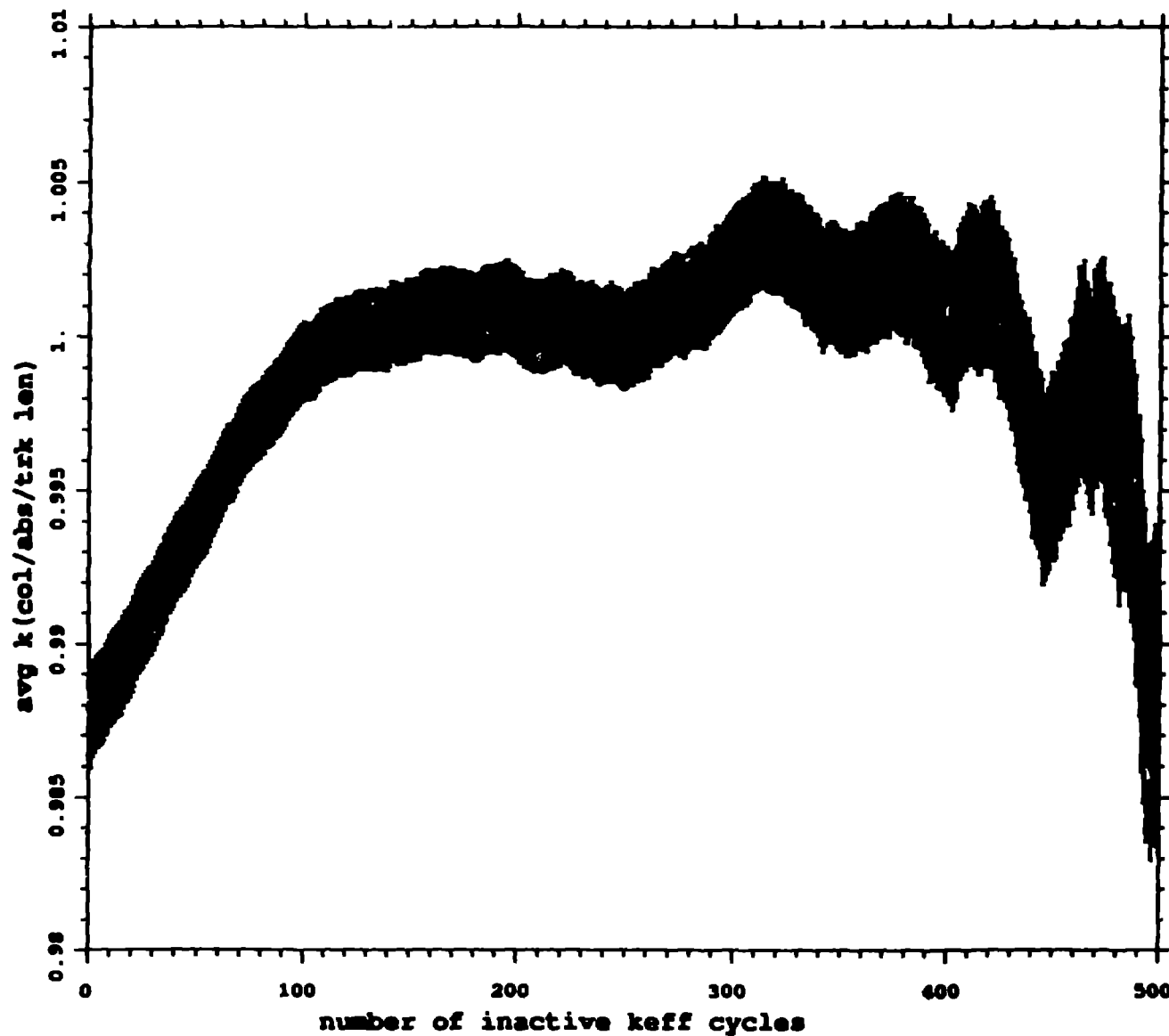
Fig. 4. One standard deviation confidence interval for the average keff of the array with Jezebel as a function of the number of cycles skipped (inactive cycles).
