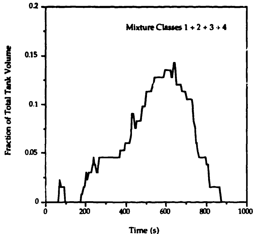
Fig. 1. Fraction of total tank dome space volume containing mixtures 1, 2, 3, and 4 for maximum expected release with inoperable ventilation system and closed riser.
