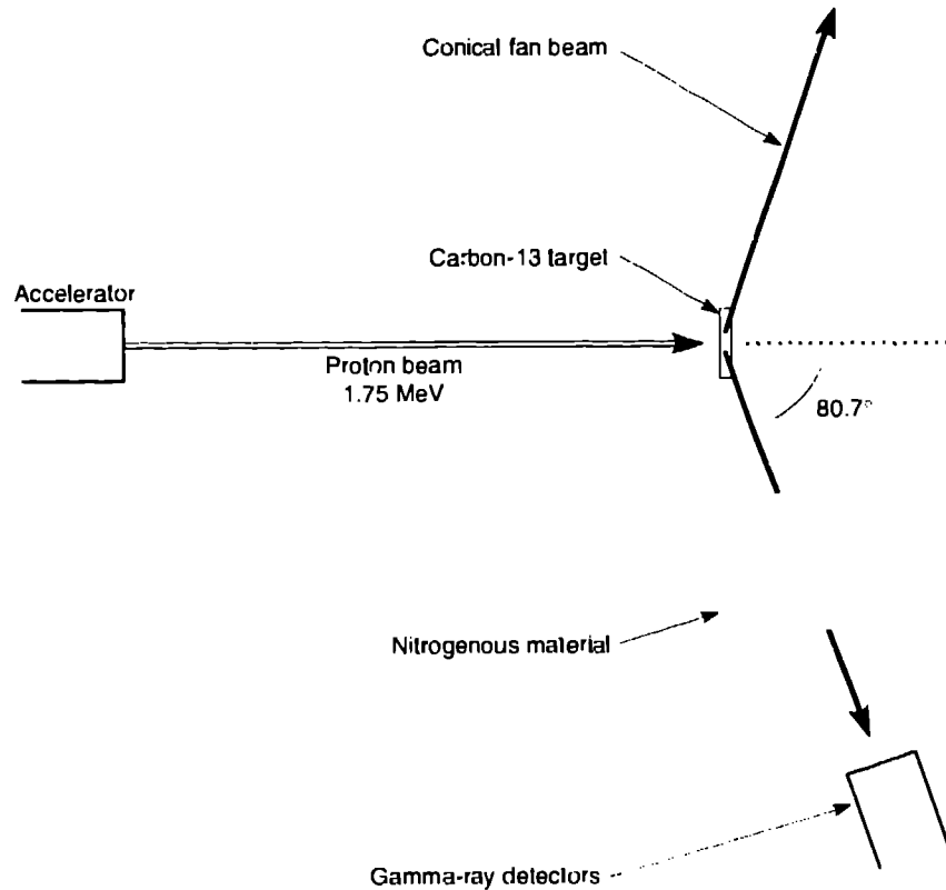
Fig. 1. Resonance-absorption-based detection concept.
