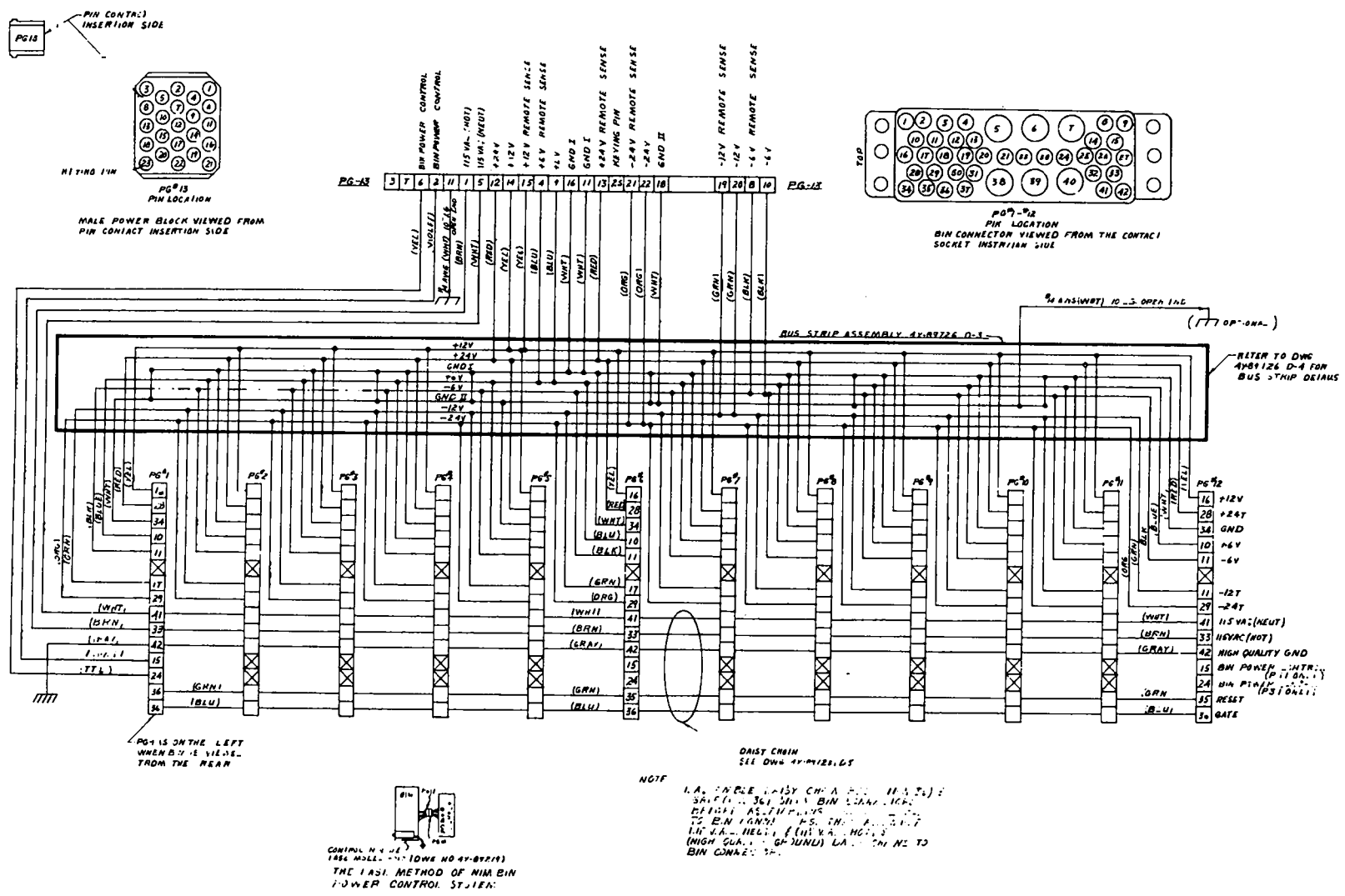
Fig. 8. 4Y-89726, D6 - Daisy chain and standard NIM bin wiring.
