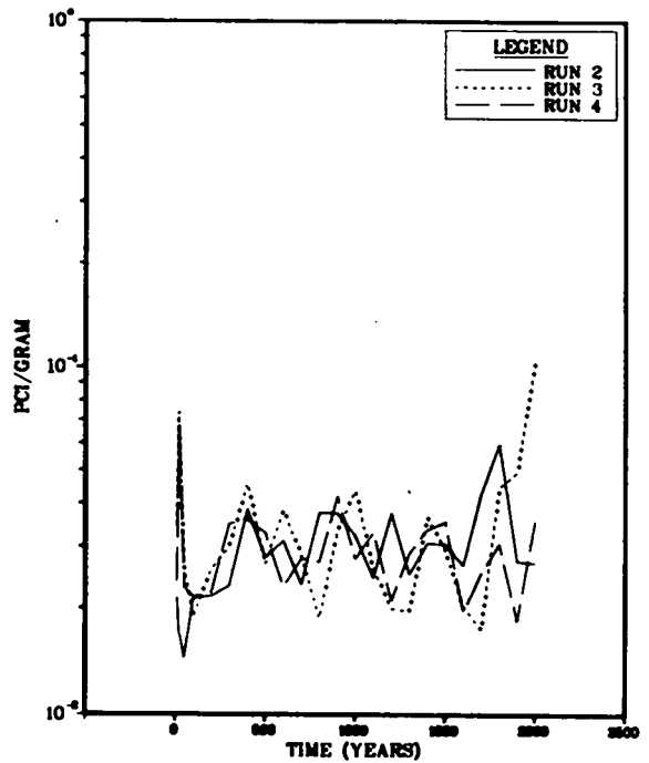
Fig. 7. Simulated concentration in above-ground biomass for piñon-juniper forest, Los Alamos, NM.
