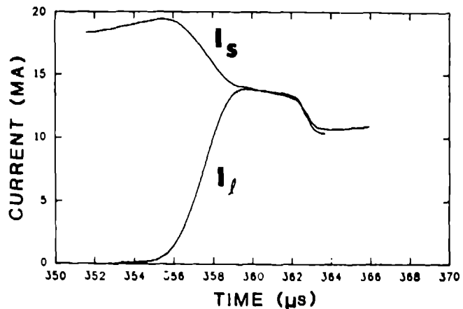
Fig. 9. I_s and I_l for Shot 1, demonstrating total current transfer with a 10-90% risetime of < 3 \mu s . In addition, the current drop at \sim 362 \mu s is due to the change in inductance as the plasma exits the gun and shows that the vacuum/dielectric interface and EFF have not failed.
