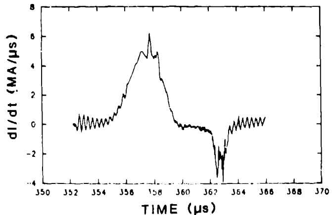
Fig. 10. Composite Faraday rotation and Rogowsky coil measurement of di/dt in the vacuum region on Shot 1. The positive spike indicates the rate of current transfer to the load, and the negative spike the effects of the pinch of gun plasma off the open end of the gun.
