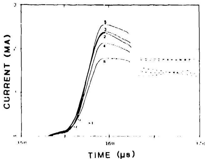
Fig. 8. Current in five of the six closing switches on Shot 1. The signal from Channel 1 went offscale due to a ground loop. The two points given show the signal strength on Channel 1 before it was lost.
