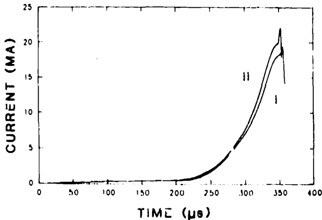
Fig. 4. Storage inductor current profiles from Shots I and II. Initial current from the capacitor bank occurs at \sim 10 \mu s , and generator crowbar occurs at \sim 155 \mu s . The spike on the peak of each waveform is due to flux compression in the EFF.
