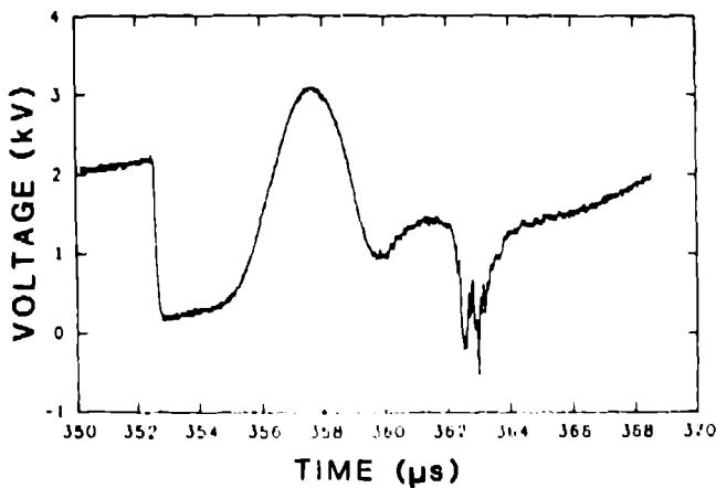
Fig. 7. Voltage across closing switches on Shot 1. The abrupt break at 352.2 \mu s occurs when the switches close. The 3\text{-kV} positive spike at 358 \mu s and the negative spikes at 363 \mu s are features due to di/dt and \sim 0.6\text{-mH} circuit inductance inside the voltage probe loop. The resistance of the switches at 360 \mu s is \sim 0.08 \text{ m}\Omega .
