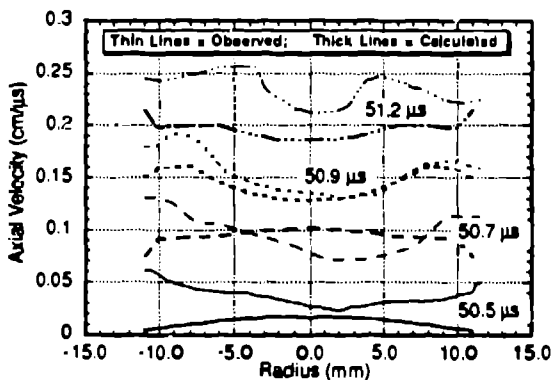
FIGURE 3 Observed and calculated axial velocity along a diameter of the plate at four times. Initial plate motion was at 50.2 \mu s.
