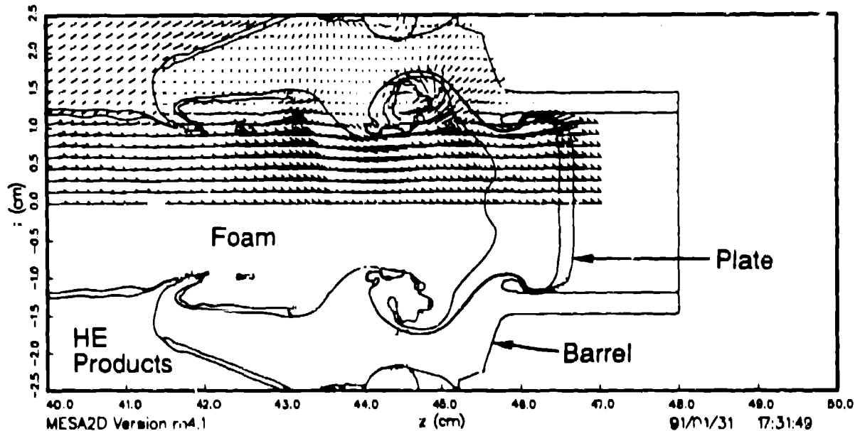
FIGURE 4 Interface plot of the barrel and plate region of the FST (from a Fig. 1b test) about 5 \mu s after start of motion of the plate. The velocity vectors represent the direction and magnitude of material velocity in every third computational cell. The maximum velocity indicated is 0.82 cm/ \mu s.
