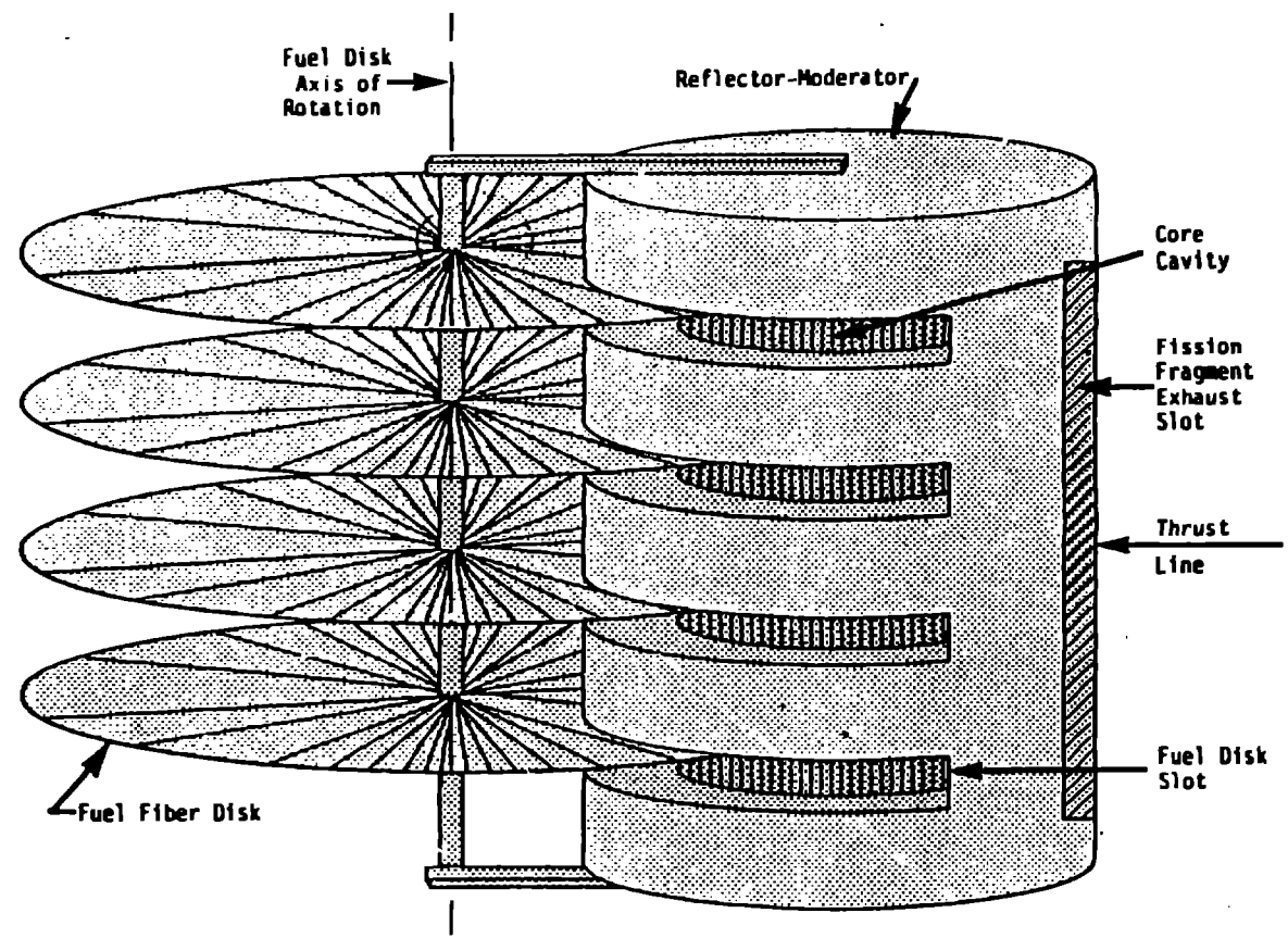
FIG. 4 Figure 4. Potential fission fragment rocket engine configuration.
