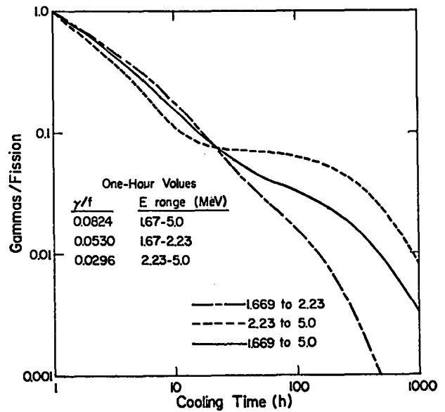
Fig. 8. Gammas per fission vs cooling time over 3 energy ranges for ^{239}\text{Pu} thermal fission.
