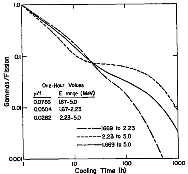
Fig. 9. Gammas per fission vs cooling time over 3 energy ranges for ^{239}\text{Pu} fast fission.
