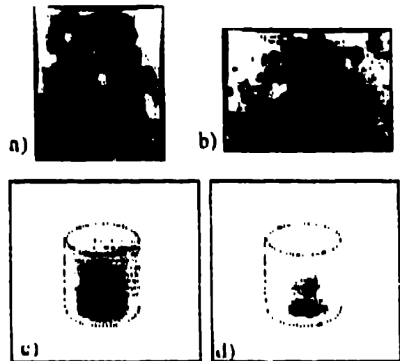
Fig. 3. Images of an electrorefining salt sample (ANL-125). (a) x-ray radiograph of the inner can showing chunks of salt. (b) x-ray radiograph of a small portion of the sample. (c) radiograph of a TGS attenuation image with 13 mm voxel size. (d) emission image at 25 mm voxel size. The radiographs of TGS images were taken with a polar angle of 60 degrees.
