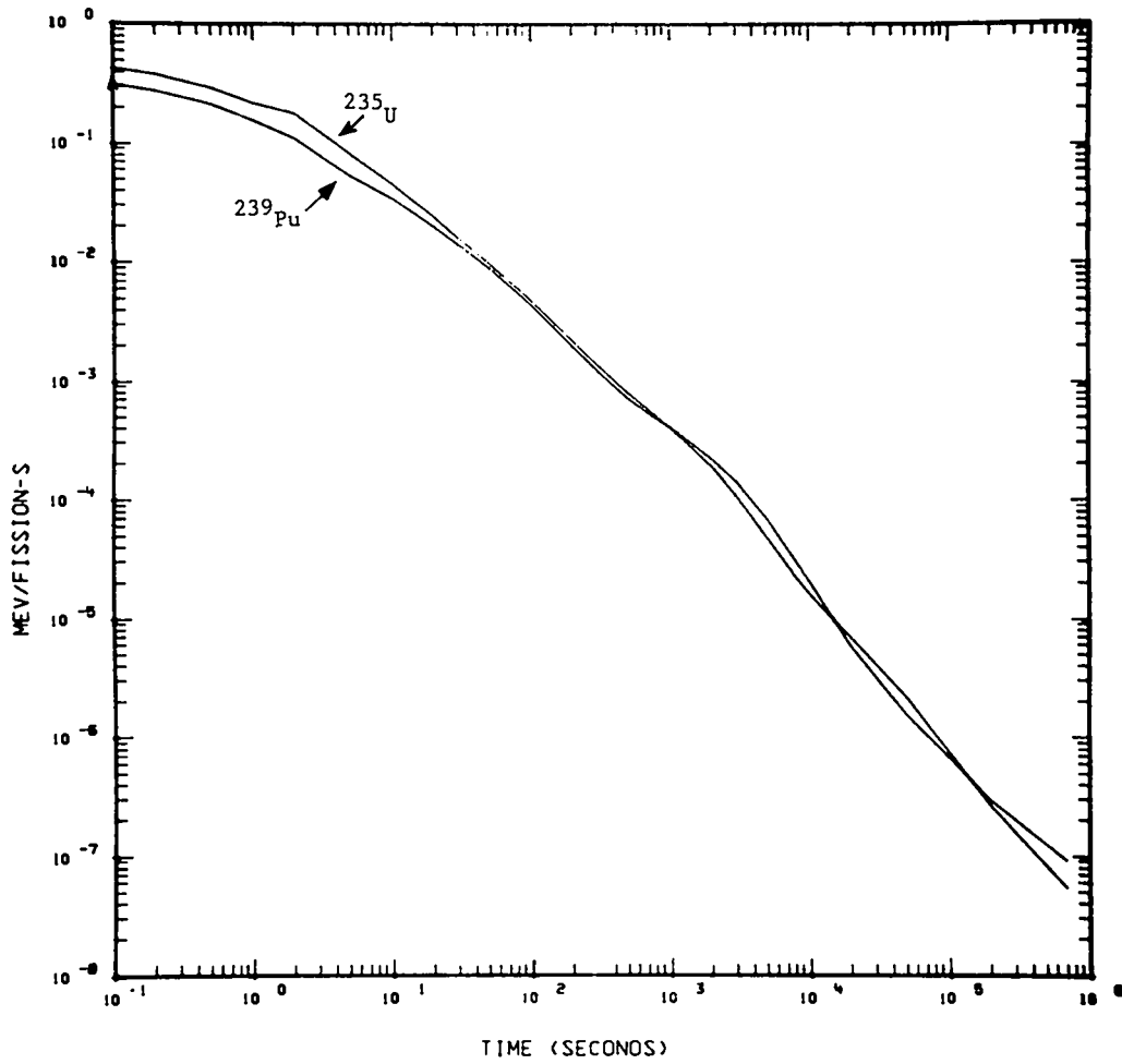
Fig. 2. 235 U and 239 Pu gamma power (MeV/fis-s) from non-gaseous fission products in fission burst.
