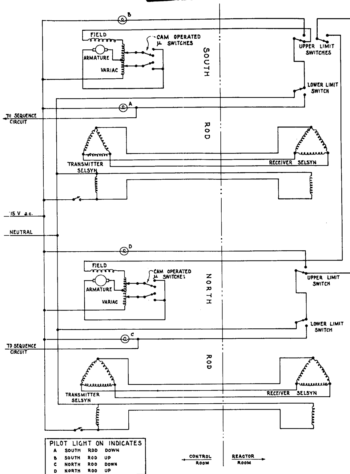
Fig. 41. Control circuit diagram.
