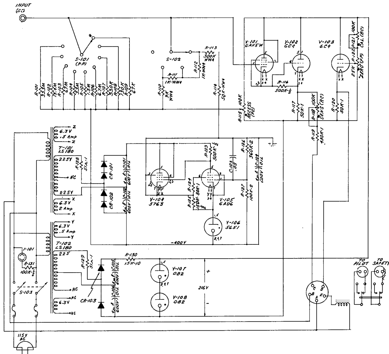
Fig. 44. Linear neutron level circuit diagram.
