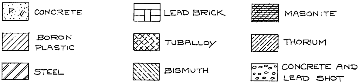
Fig. 2. Cross section through the reactor.
