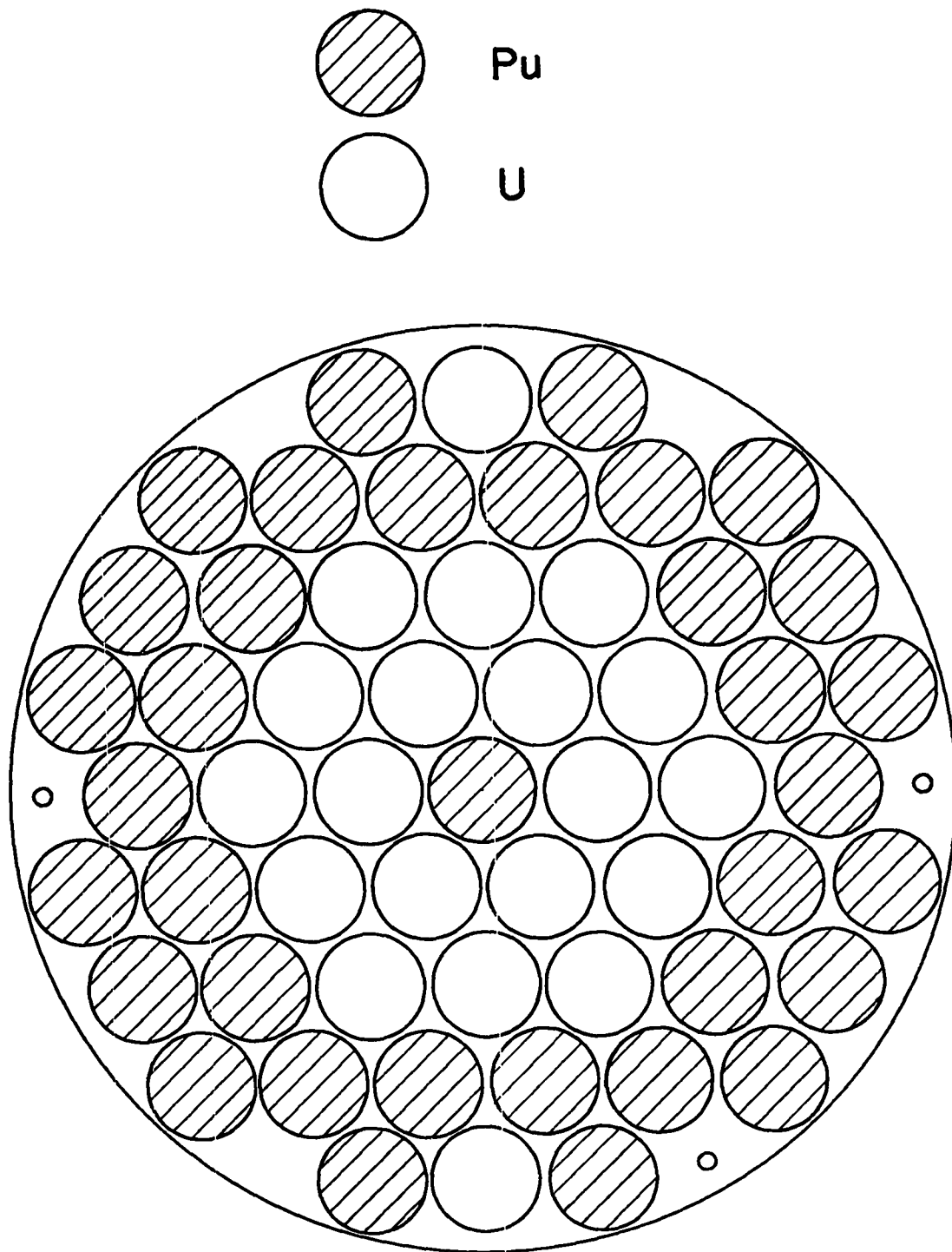
Fig. 48. Reactor fuel loading (peripheral).
