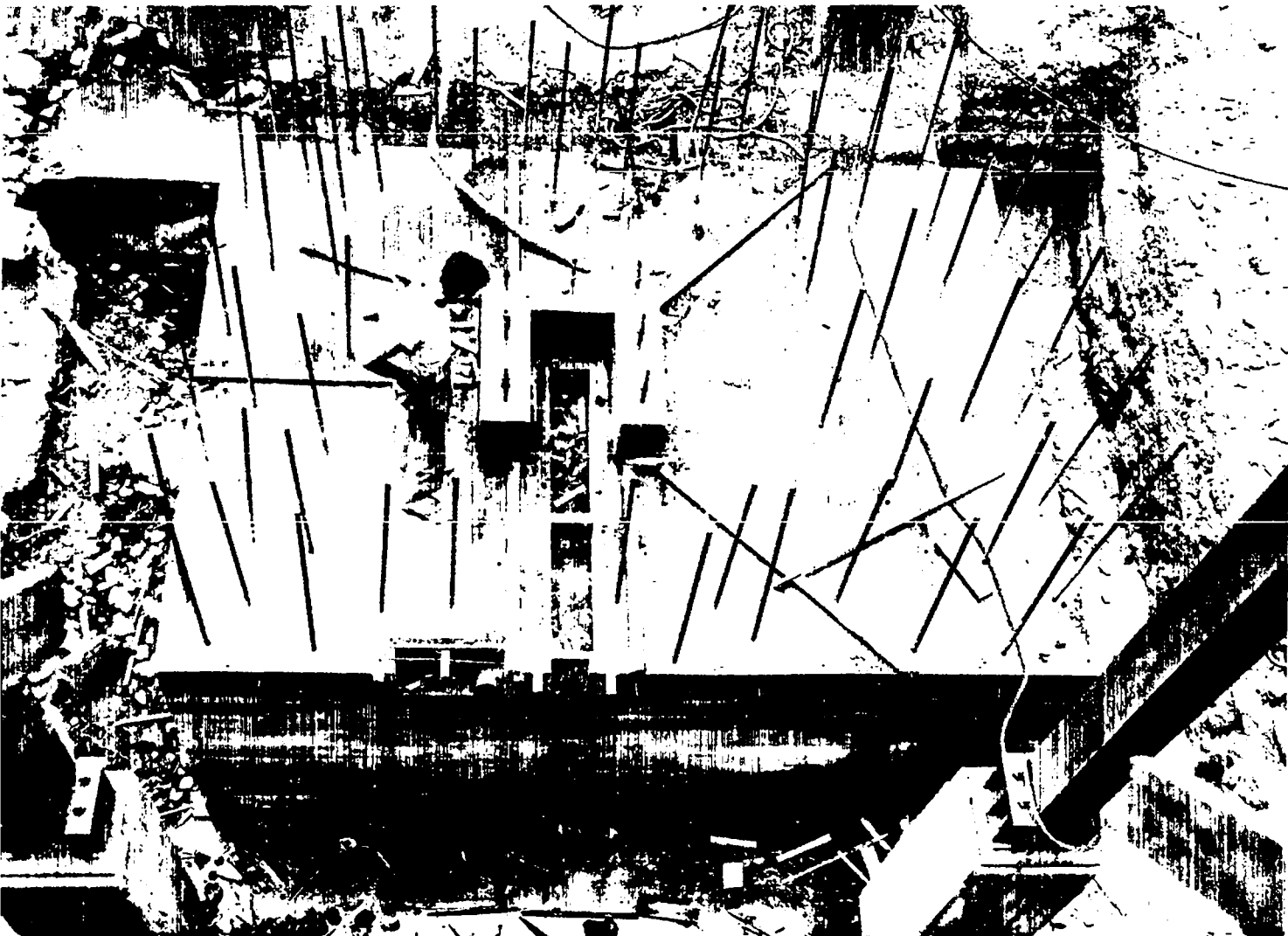
Fig. 5. Reactor foundation.
