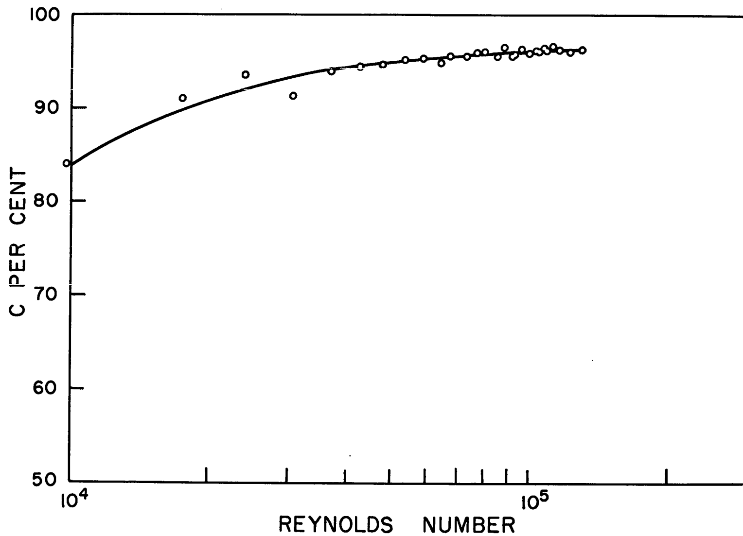
Fig. 32. Venturi calibration.
