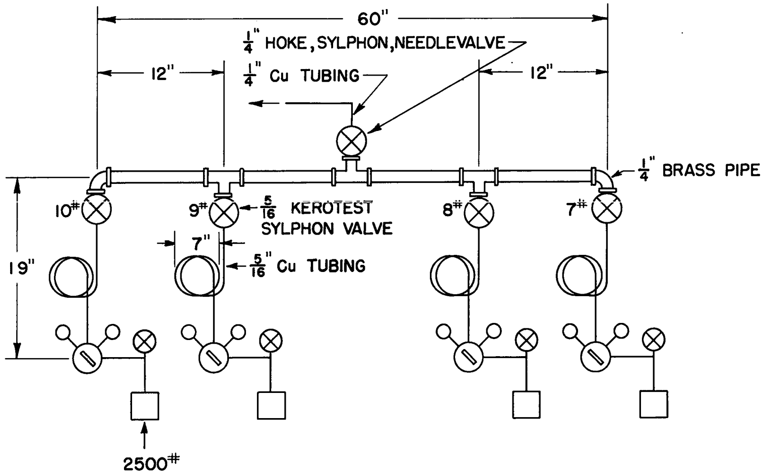
Fig. 34. Helium supply manifold.
