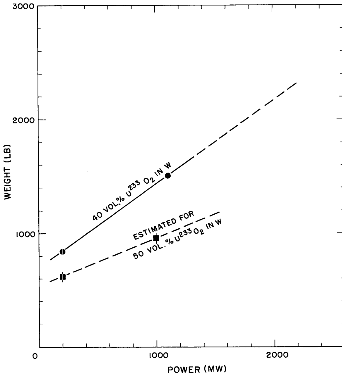
Fig. 4 Reactor weight vs. power for U^{233}O_2 -W reactors. Reactor weight = core + reflector + pressure shell + \approx 100 lb miscellaneous.
