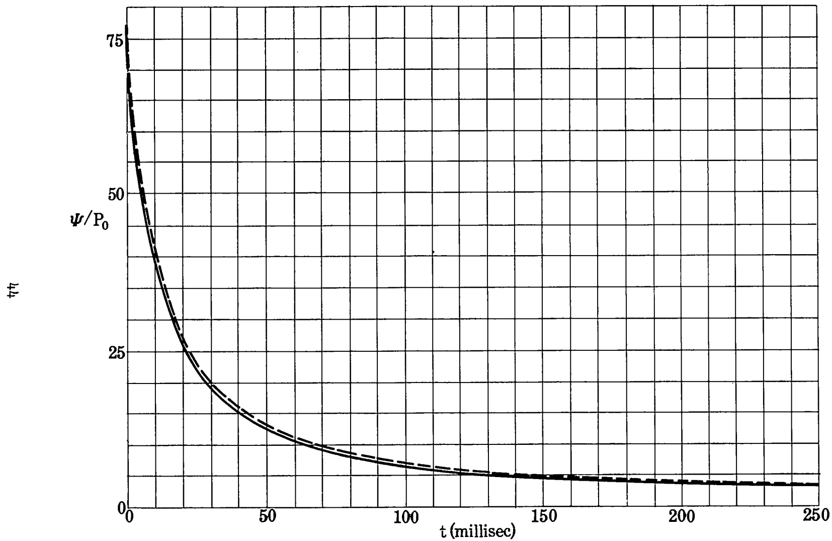
Fig. 11. Shock pressure as a function of time; ——— Problem M, - - - Problem Herman
