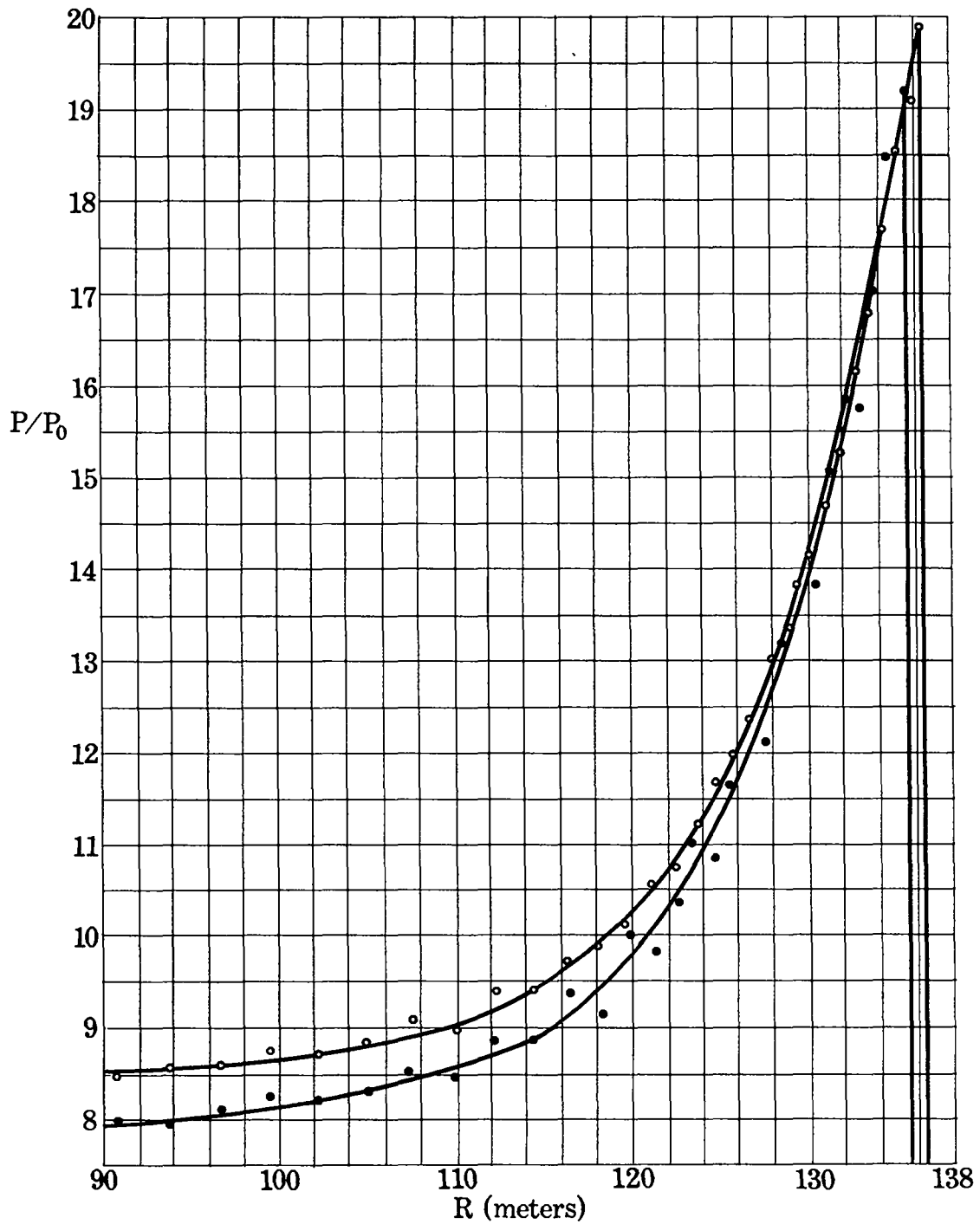
Fig. 4. Pressure as a function of the Eulerian radius at t = 30 milliseconds; \bullet Problem M, \circ Problem Herman
