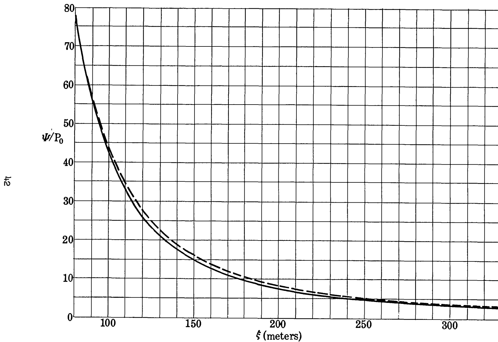
Fig. 9. Shock pressure as a function of shock position; — Problem M, - - - Problem Herman
