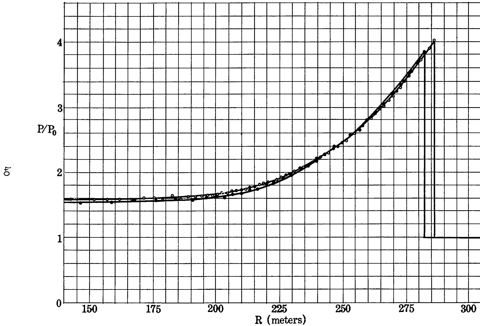
Fig. 7. Pressure as a function of the Eulerian radius at t = 200 milliseconds; • Problem M, ◦ Problem Herman
