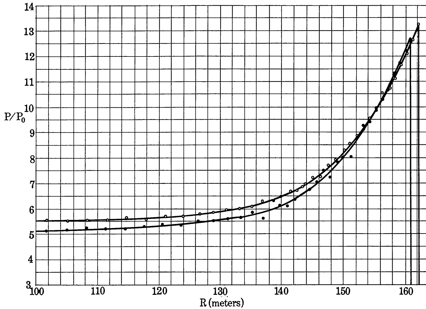
Fig. 5. Pressure as a function of the Eulerian radius at t = 50 milliseconds; • Problem M, ○ Problem Herman
