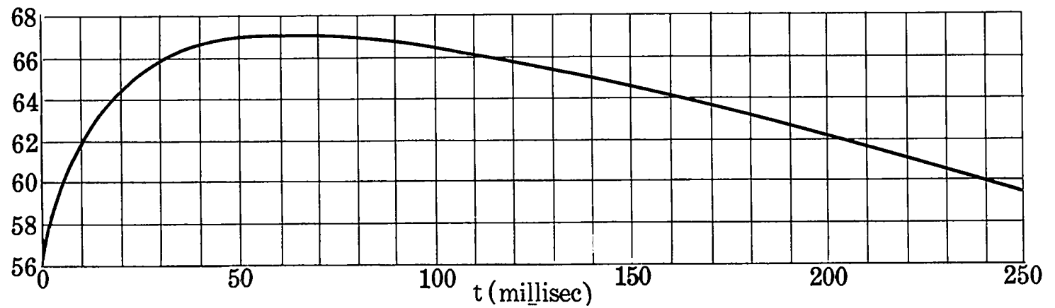
Fig. 15. Total kinetic energy as a function of time
