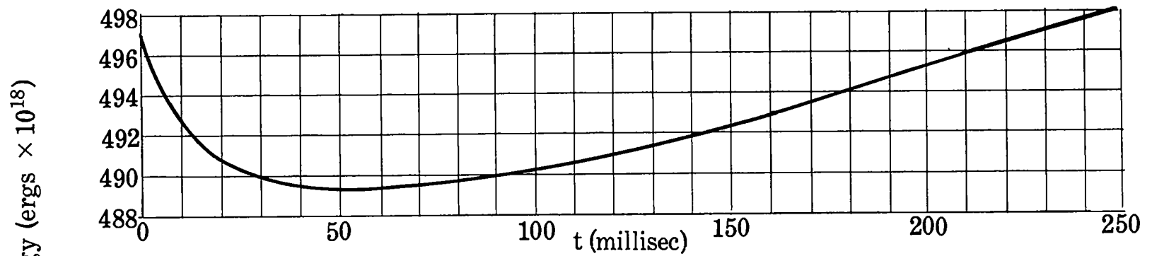
Fig. 14. Total internal energy as a function of time
