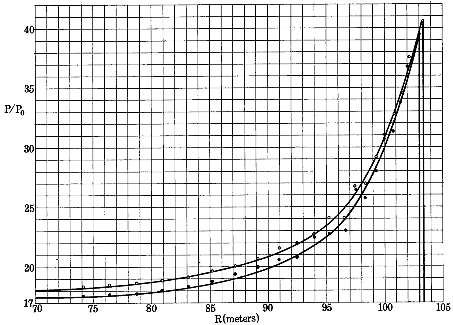
Fig. 3. Pressure as a function of the Eulerian radius at t = 10 milliseconds; • Problem M, ◦ Problem Herman
