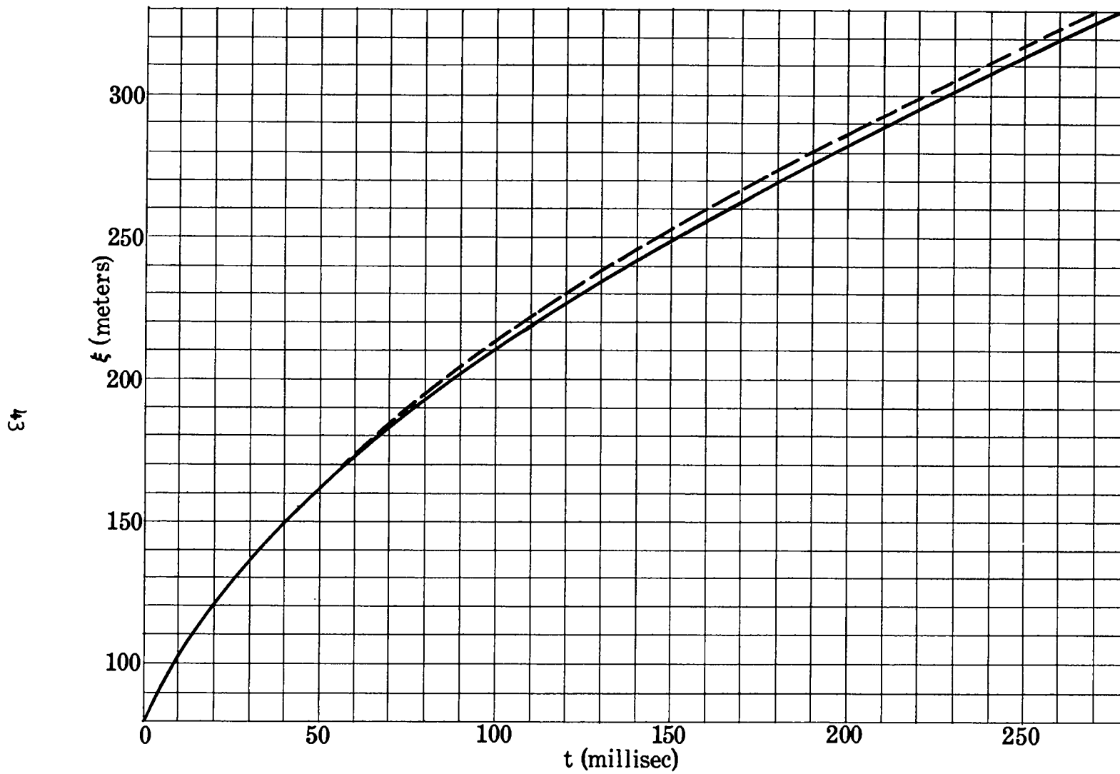
Fig. 10. Shock position as a function of time; ——— Problem M, - - - Problem Herman
