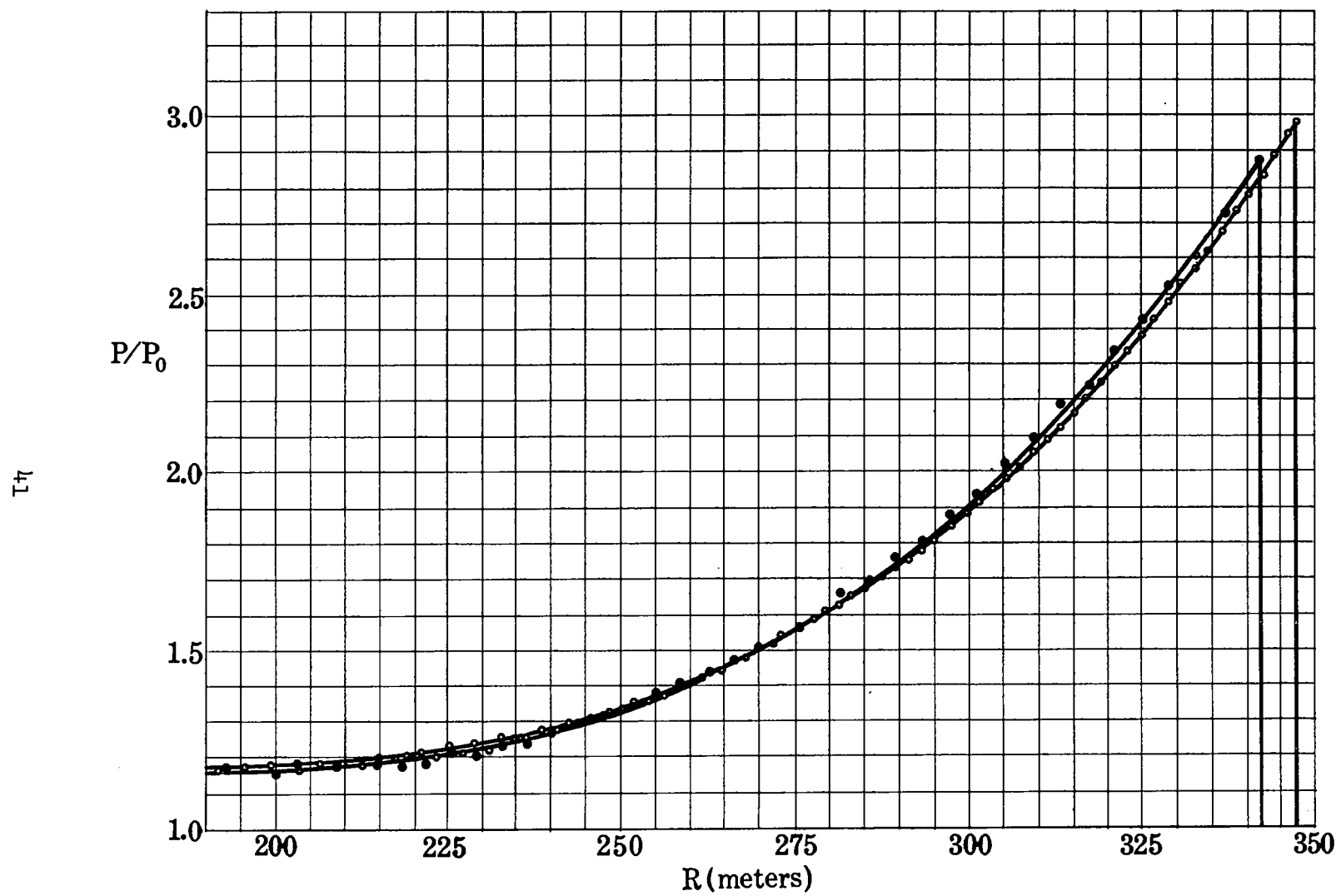
Fig. 8. Pressure as a function of the Eulerian radius at t = 300 milliseconds; • Problem M, ° Problem Herman
