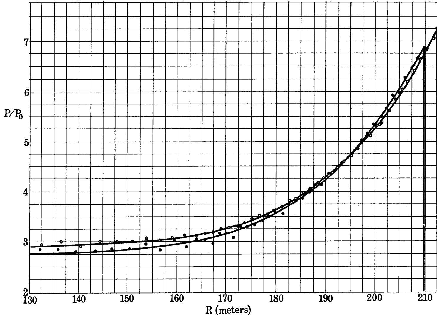
Fig. 6. Pressure as a function of the Eulerian radius at t = 100 milliseconds; \bullet Problem M, \circ Problem Herman
