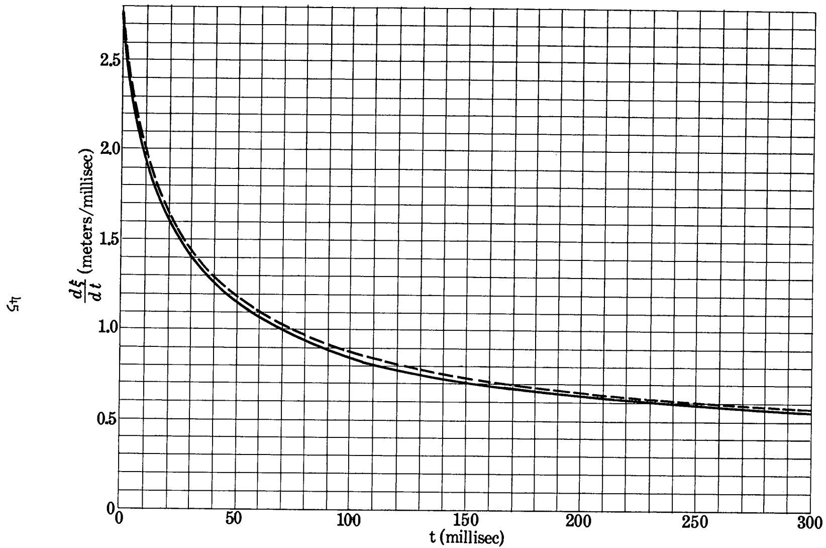
Fig. 12. Shock velocity as a function of time; — Problem M, - - - Problem Herman
