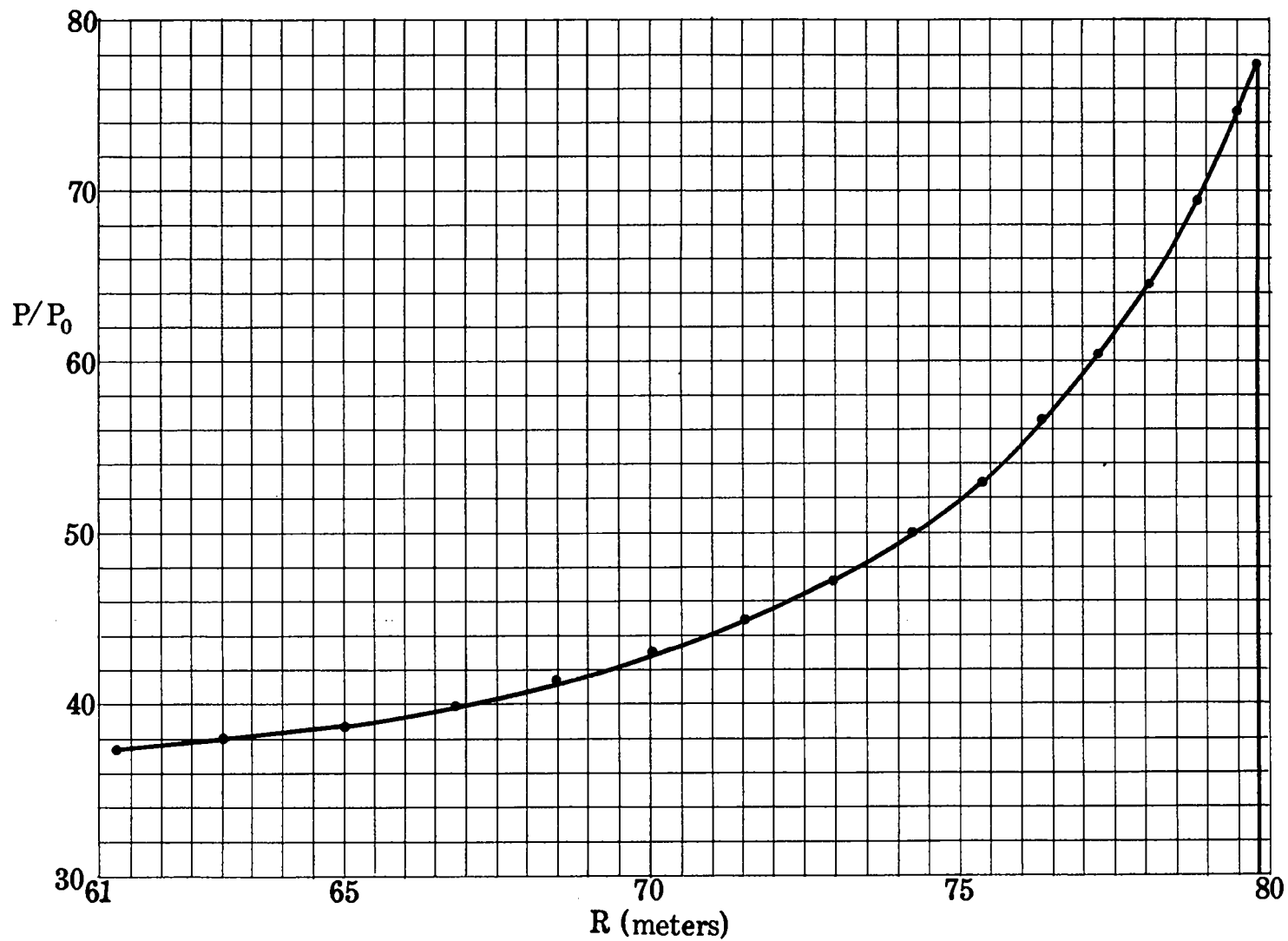
Fig. 2. Pressure as a function of the Eulerian radius at t = 0 milliseconds for both Problem M and Problem Herman
