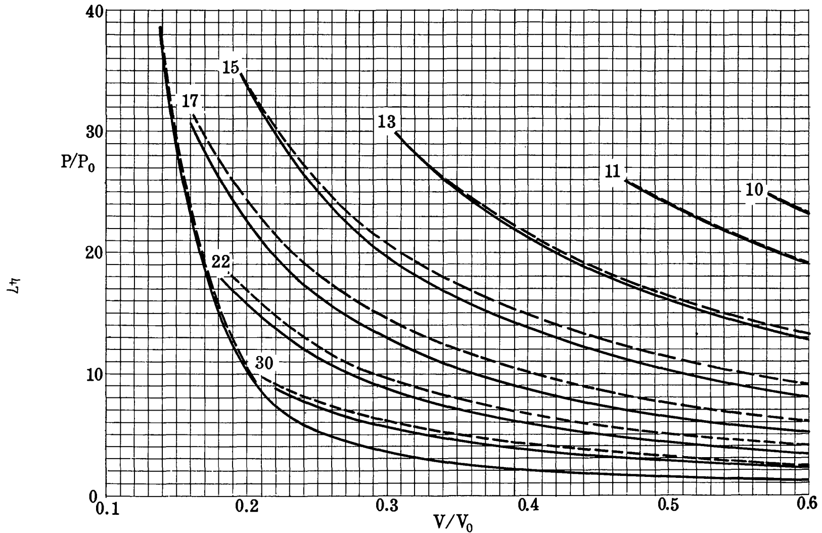
Fig. 16. The Hugoniot curve and some adiabatic curves in the pressure-volume plane; ——— Problem M, - - - Problem Herman
