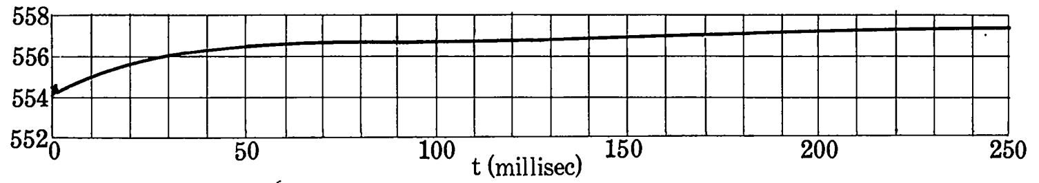
Fig. 13. Total energy as a function of time
