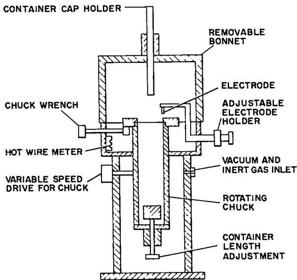
Fig. 4. Welding fixture schematic.
