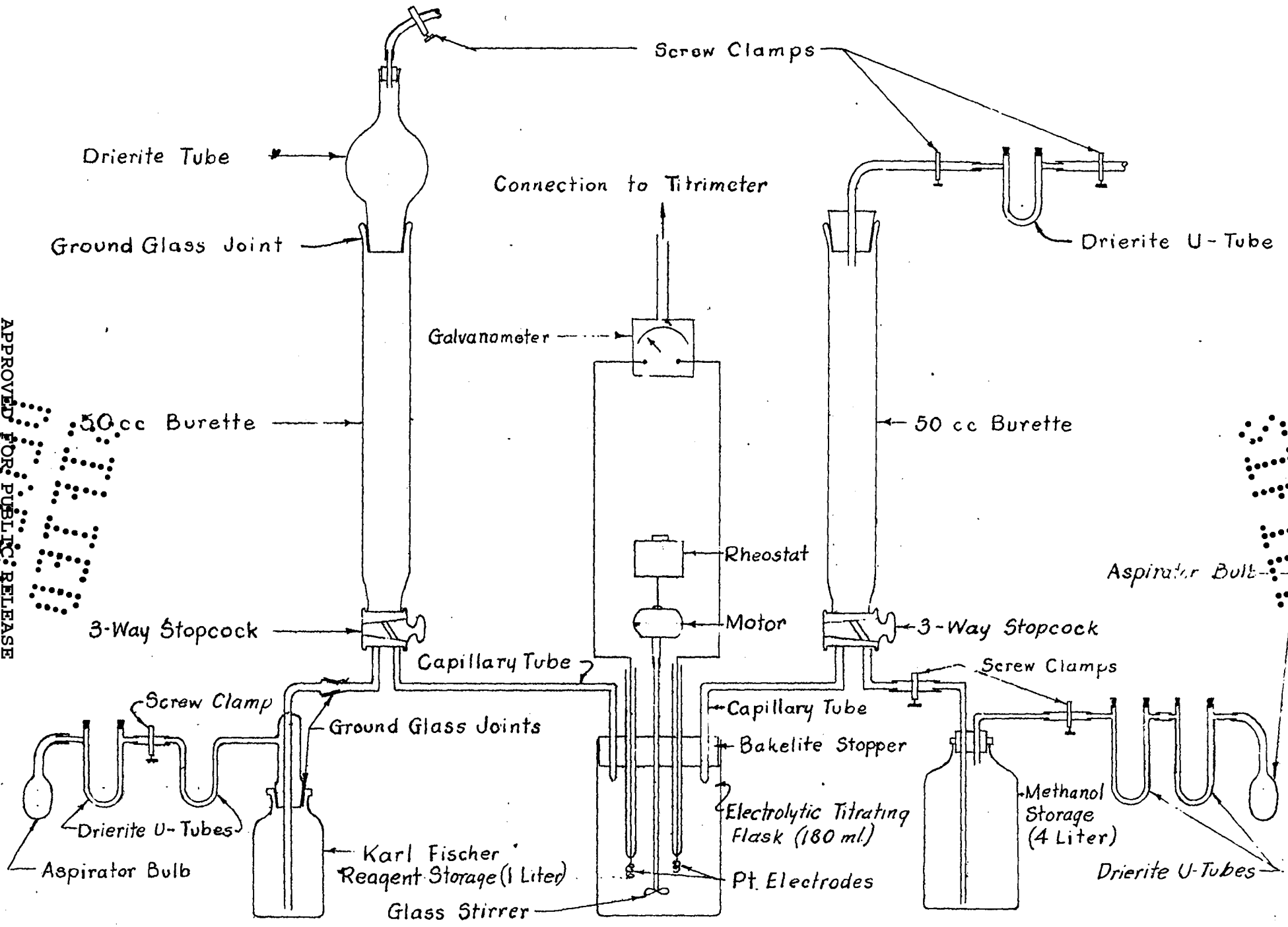
FIG. 1 DIAGRAM OF WATER-DETERMINATION ASSEMBLY
