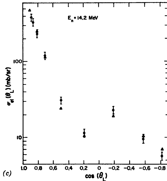
Fig. 4. Comparison of the present differential elastic cross section ( \bullet ) and the ENDF/B IV differential elastic cross section ( \blacktriangle ) for (a) 5.9-MeV, (b) 10.1-MeV, and (c) 14.2-MeV incident neutrons on beryllium. The laboratory cross sections are plotted as a function of the cosine of the laboratory scattering angle. The total errors are plotted. See text for more details on the errors.
