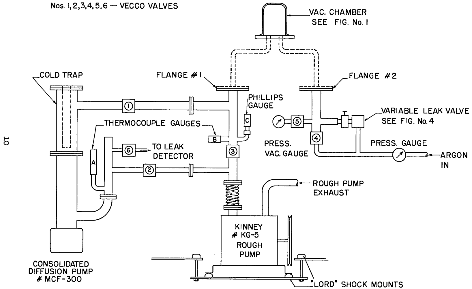
Fig. 2. Schematic diagram of vacuum system.
