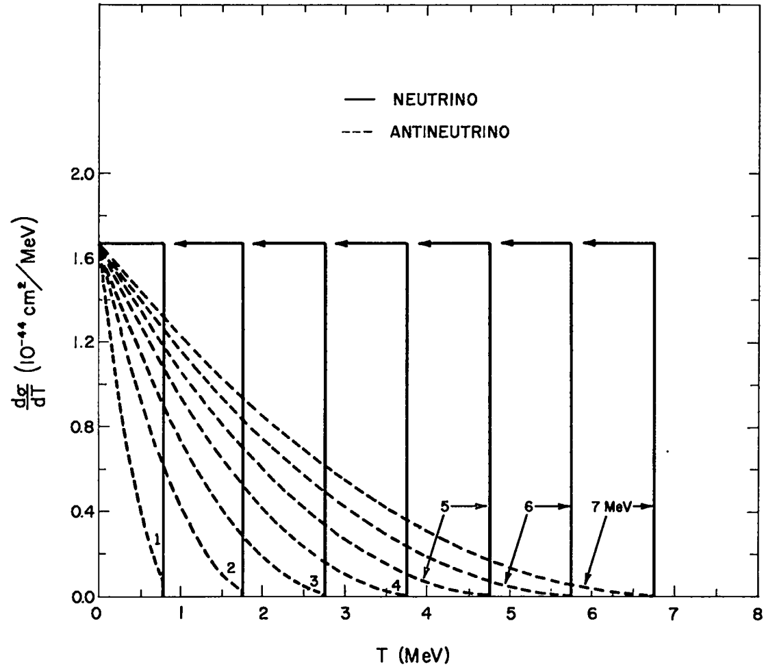
Figure I. Laboratory differential cross section per unit electron recoil kinetic energy T , vs T , for elastic neutrino and antineutrino scattering on electrons. The curves are labeled by the incident neutrino or antineutrino laboratory energy in MeV. Note that the electron recoil spectrum is flat from T = 0 to T_{\text{max}} for the case of incident neutrinos. The calculation assumes that there are no neutral symmetric currents.
