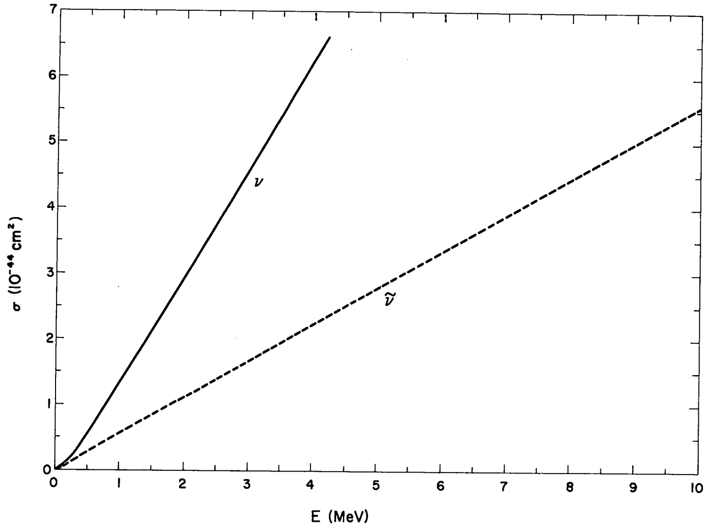
Figure II. Total cross section for elastic neutrino and antineutrino scattering on electrons vs the incident neutrino or antineutrino laboratory energy. The calculation assumes that there are no neutral symmetric currents.
