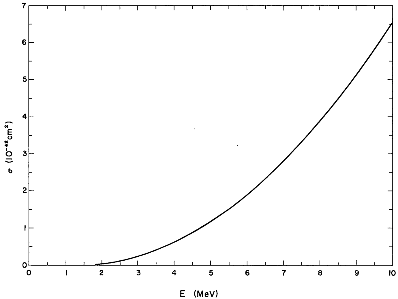
Figure III. Total cross section for \bar{\nu} + p \rightarrow n + e^+ vs the incident antineutrino laboratory energy. The anisotropy (which is less than 8%) is given in the text.
