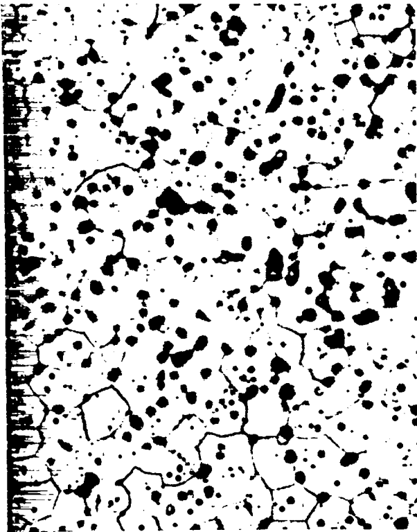
^{239}\text{PuO}_2 (10.2 g/cc)
