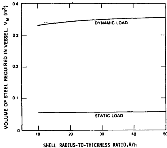
Fig. 5. Volume of vessel material required to contain 8.16 kg of PBX-9404 as a function of vessel radius-to-thickness ratio for a steel vessel ( \epsilon_{yield} = 0.0011 , \rho_o = 1 \text{ kg/m}^3 ).
