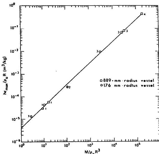
Fig. 4. Experimental data plotted in terms of scaling law variables. Numbers adjacent to data points indicate the value of initial air density in the vessel; 1 is \rho_0 = 1 kg/m 3 , 2 is \rho_0 = 0.1 kg/m 3 , 3 is \rho_0 = 1 \times 10^{-3} , 4 is \rho_0 = 5 \times 10^{-5} kg/m 3 .
