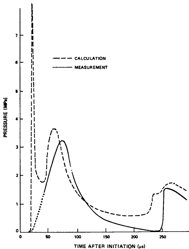
Fig. 13. Comparison of measured and calculated pressure acting on the vessel wall ( \rho_0 = 1 g/m 3 vacuum case, other parameters in- dicated in Fig. 6a).
