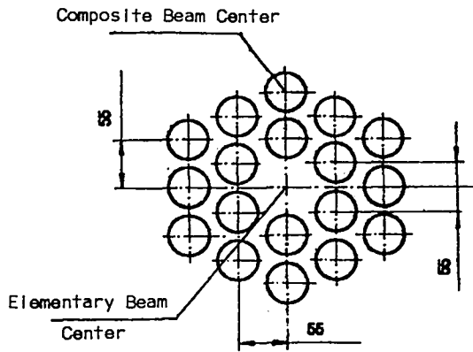
Fig. 13. Composite beam structure.
