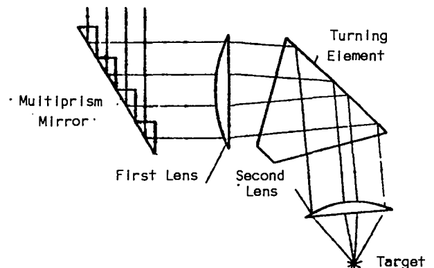
Fig. 15. The two-lens modular focusing system.
