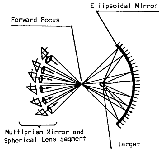
Fig. 17. Operating principle of ellipsoidal mirrors.
