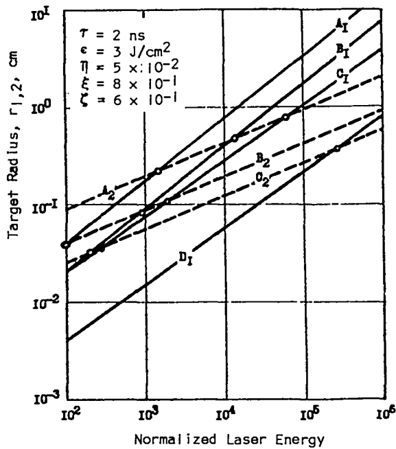
Fig. 2. Comparison of dependences of limiting values r_1 (—) and r_2 (---) of target radius on laser energy for facilities with rod ( m = 10 ; D_0 = 45 mm) and disc ( m = 34 , D_0 = 300 mm) active elements. A_1 is m = 34 , D_0 = 300 mm, \Delta N = 1 ; B_1 is m = 34 , D_0 = 300 mm, \Delta N = 0.5 ; C_1 is m = 10 , D_0 = 45 mm, \Delta N = 0.5 ; D_1 is m = 10 , D_0 = 45 mm, \Delta N = 0.1 ; A_2 is \gamma = 5 \times 10^{-3} ; B_2 is \gamma = 5 \times 10^{-2} ; and C_2 is \gamma = 2 \times 10^{-1} .
