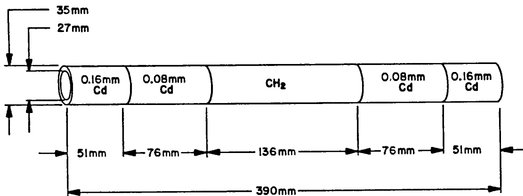
Fig. 5. Schematic diagram of 4-mm-thick CH 2 sleeve and cadmium wrap.
