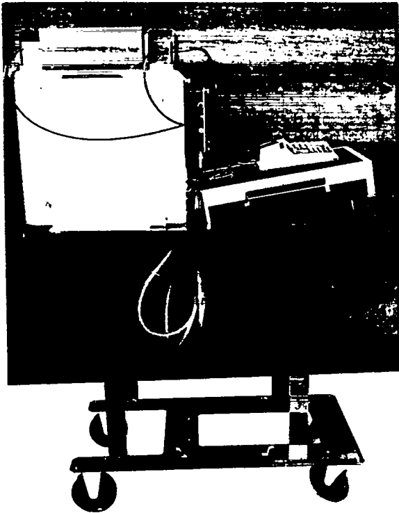
Fig. 3. Photograph of the complete Passive Coincidence Collar, including detector head, IRT Model HEC-100 coincidence electronics, HP-97 calculator, and support cart.
