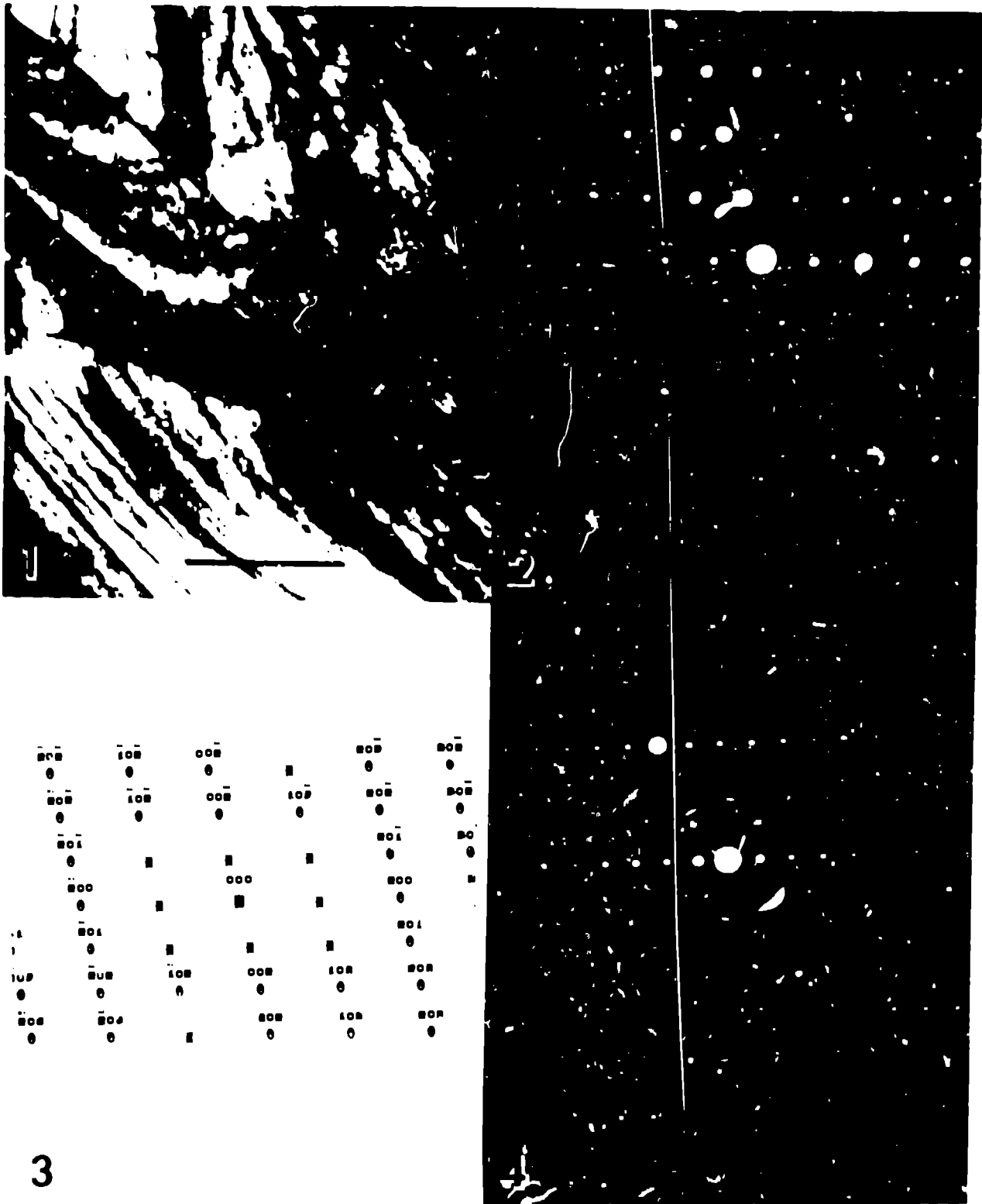
Fig 1.--Grain boundaries in \alpha -Pu. Bar = 0.25 \mu m. Fig 2.--SAD of \alpha -Pu, (020). Fig 3.--Calculated diffraction pattern (020). Fig 4.--SAD of \alpha -Pu (001) showing \text{PuO}_2 oxide trace.
