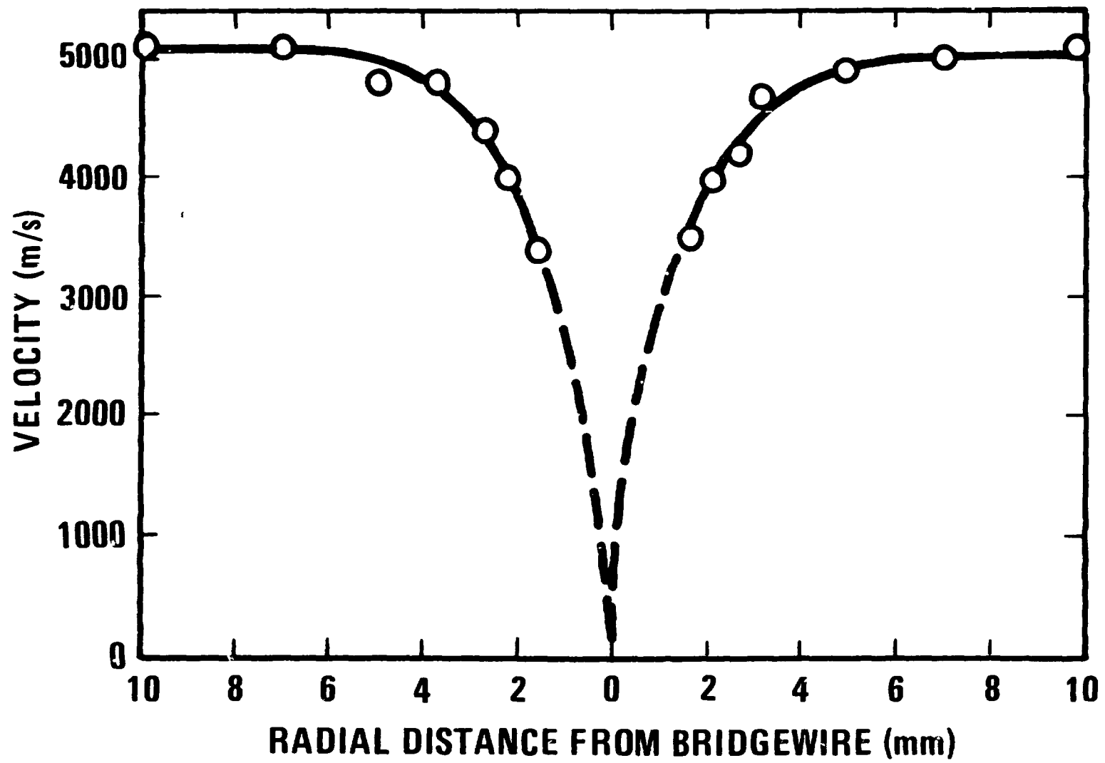
Fig. 5 Radial buildup to detonation. Firing voltage = 4000 V
