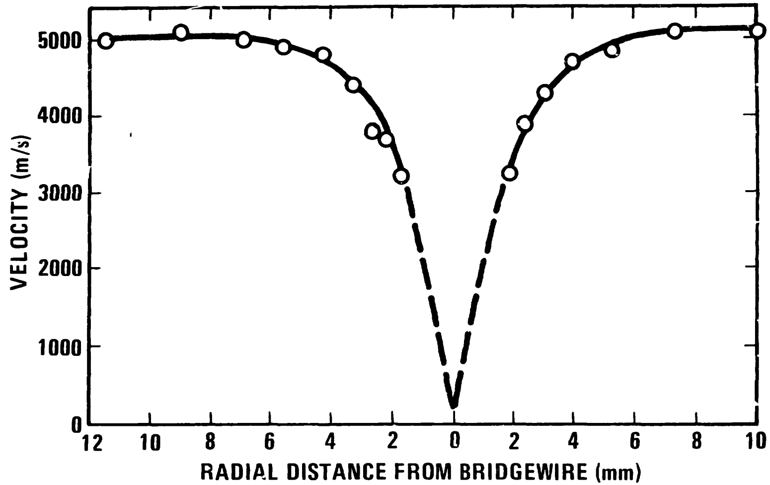
Fig. 4 Radial buildup to detonation. Firing voltage = 1300 V
