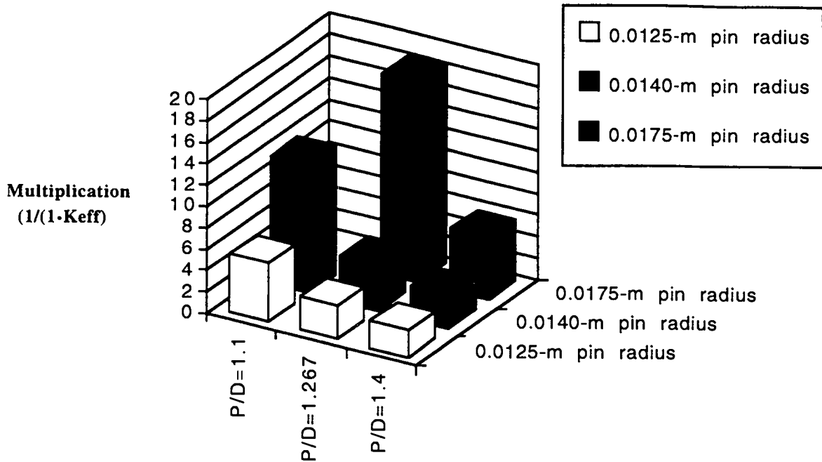
Figure 5-6. Neutron multiplication for various pitch-to-diameter ratios and pin radii (12X12 array of molybdenum/stainless-steel-clad pins).
