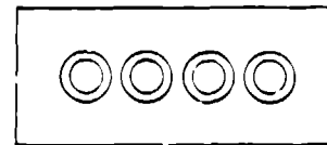
MORE COMPACT - SEPARATE REACTORS IN SINGLE CONTAINMENT CELL Reduced Clearance Between Reactors Some Clearance Around Reactors Linear Array
