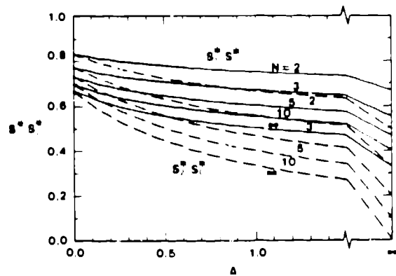
Fig. 6. Compact multicavity blanket concept total outer surface area savings relative to conventional separate blankets ( S^*/S_0^* ) for the geometry of Fig. 2.
