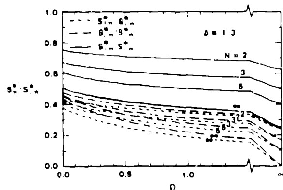
Fig. 9. Compact multireactor containment-cell total wall area ( S^*/S_0 ) savings relative to conventional cells.
