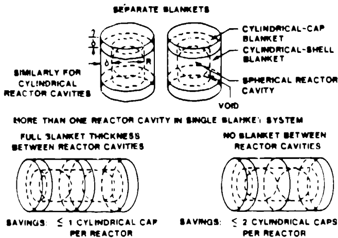
Fig. 3. Transformation of separate spherical (or cylindrical) reactor cavity/cylindrical-shell blanket combinations into linear multicavity cylindrical-shell blanket concepts.
