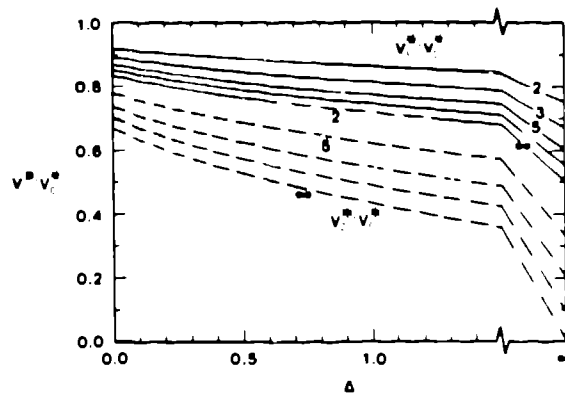
Fig. 5. Compact multicavity blanket concept total volume savings relative to conventional separate blankets ( V^*/V_0^* ) as function of reduced blanket thickness ( \Delta = \delta/R ) and number of reactor cavities ( N ) for the geometry of Fig. 2.
