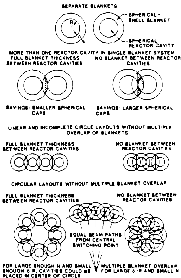
Fig. 4. Transformation of separate spherical reactor cavity/spherical-shell blanket combinations into linear and circular multicavity spherical-shell blanket concepts.
