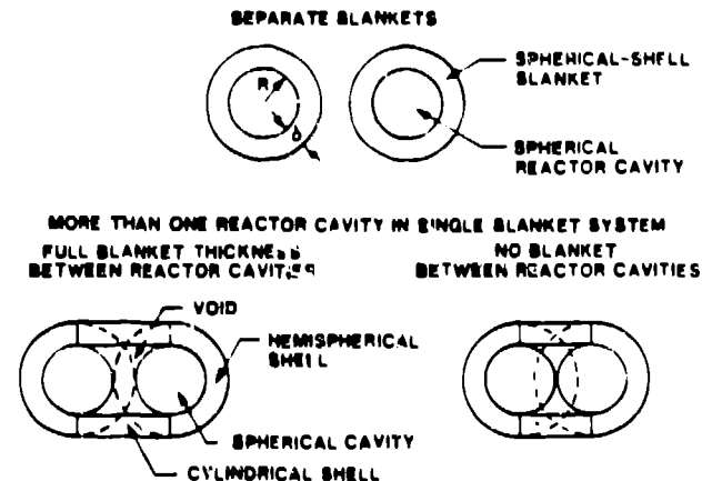
Fig. 2. Transformation of separate spherical reactor cavity/spherical-shell blanket combinations into linear multicavity cylindrical-shell/hemispherical-shell blanket concepts.
