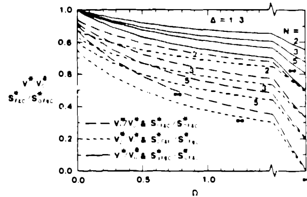
Fig. 8. Compact multireactor containment-cell concept total volume ( V^*/V_0 ) and floor and ceiling area ( S_{\text{floor}}^*/S_{\text{floor},0} ) savings relative to conventional single-reactor cells as functions of reduced clearance around reactors ( \Omega = r/(R + r) ) and number of reactor cavities ( N ) for a fixed representative value of reduced blanket thickness ( \Delta = \delta/R ).
