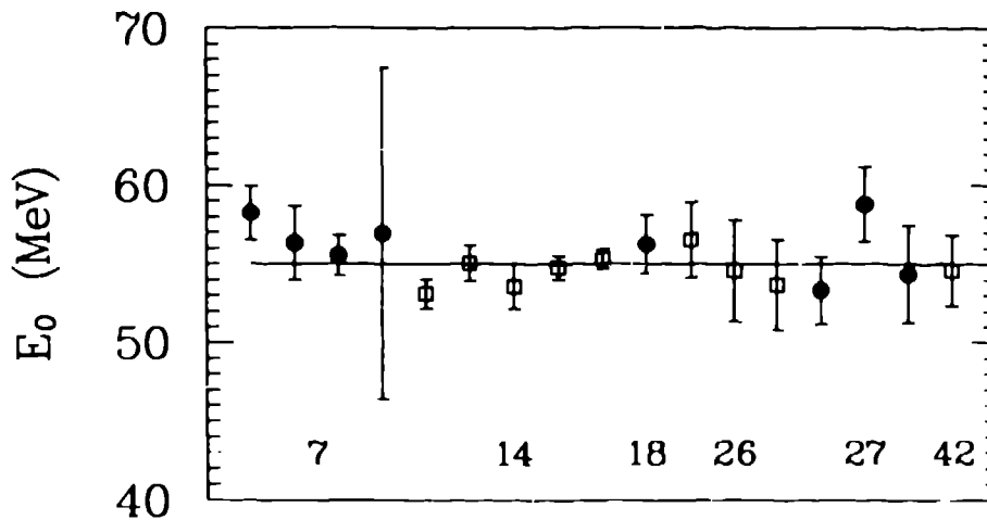
Fig. 4 The parameter E_0 = E_p/(\sigma_{GT}/\sigma_F)^{1/2} . Solid circles are alternated with open squares to indicate data points for different nuclides. For a given nuclide, the bombarding energy increases from left to right. From the left, the data correspond to ^7\text{Li} , ^{11}\text{C} , ^{13}\text{C} , ^{14}\text{C} , ^{18}\text{O} , ^{26}\text{Mg} , ^{27}\text{Al} , and ^{42}\text{Ca} . The solid horizontal line represents the weighted average E_0 = 55.0 \pm 0.4 .
