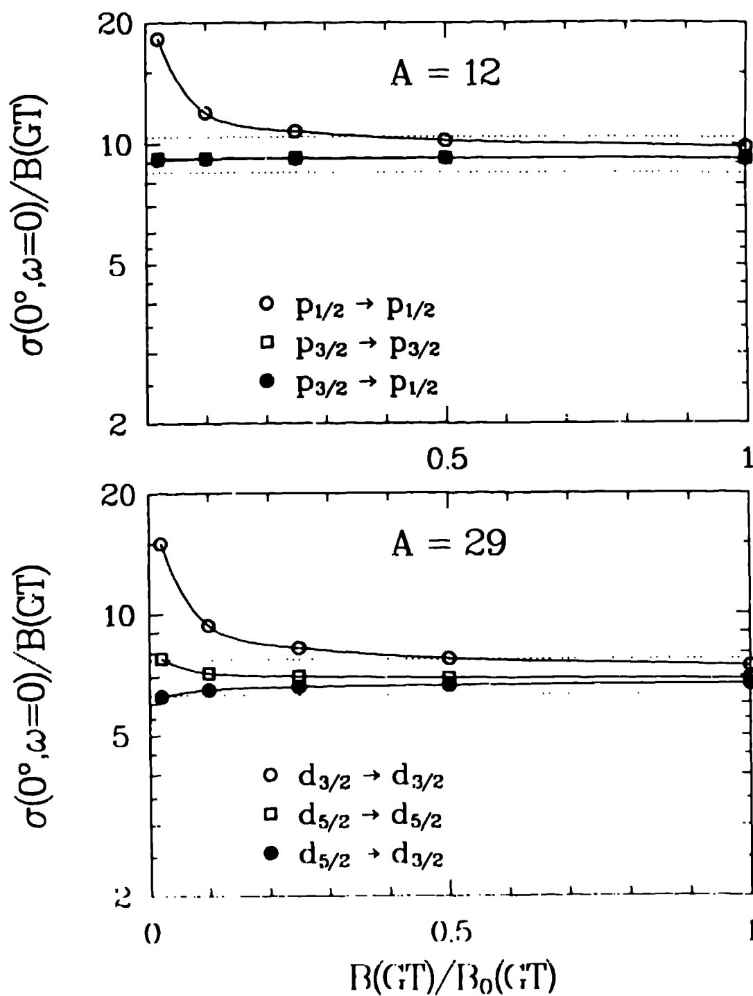
Fig. 2 Values of the GT unit cross section for A-12 and A-29. Starting with the three pure single particle transitions indicated ( B(\text{GT})/B_0(\text{GT}) = 1 ), the GT amplitude was decreased while holding the other amplitudes fixed. B_0(\text{GT}) represents the full single particle strength. The dotted horizontal lines indicate a 10% variation from the average value at B(\text{GT})/B_0(\text{GT}) = 1 . The FL 175 MeV interaction containing central, spin orbit, and tensor terms was used in the calculations.
