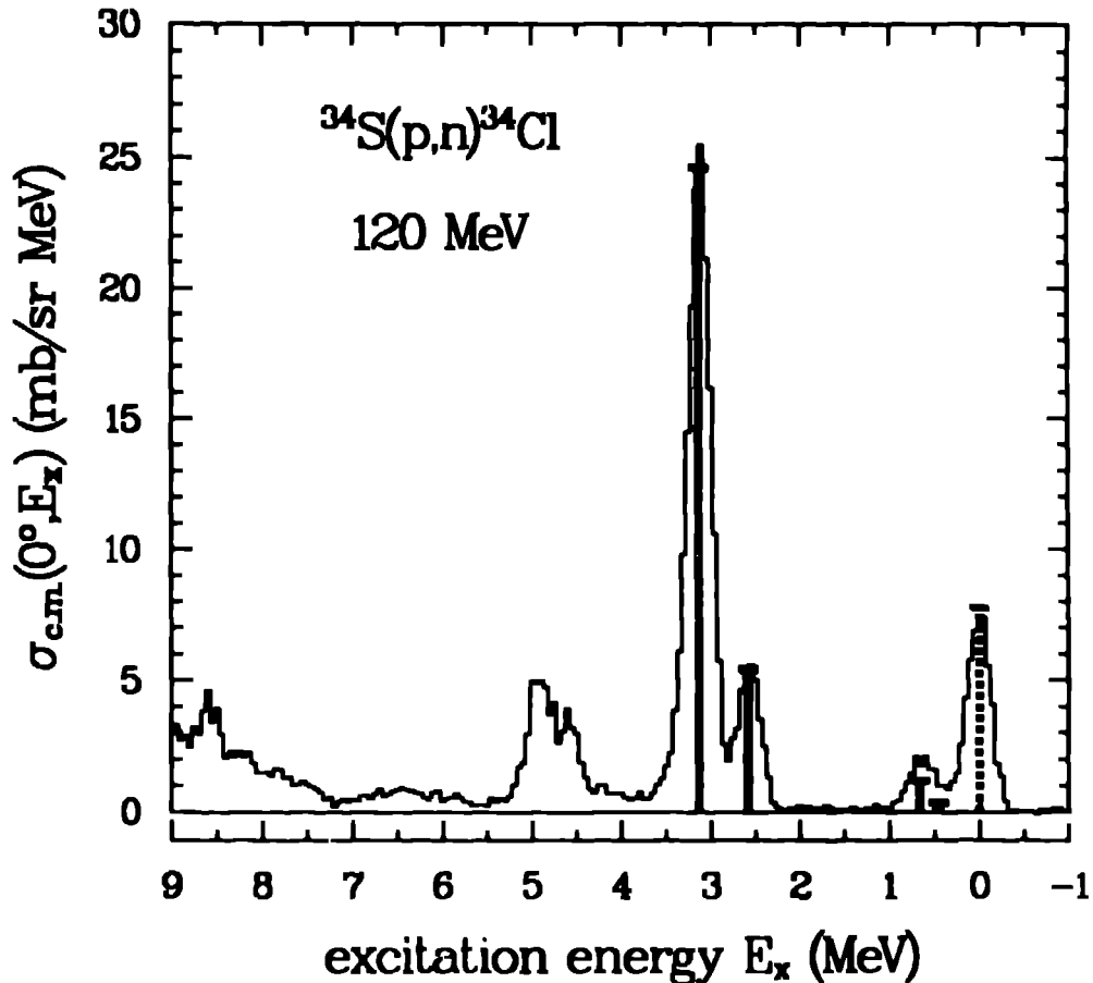
Fig. 8 Cross section spectrum for ^{34}\text{S}(p,n) at 0^\circ and 120 MeV. The vertical bars represent the GT transition strengths for analogous beta decays. The Fermi strength is indicated by the dashed vertical line.
