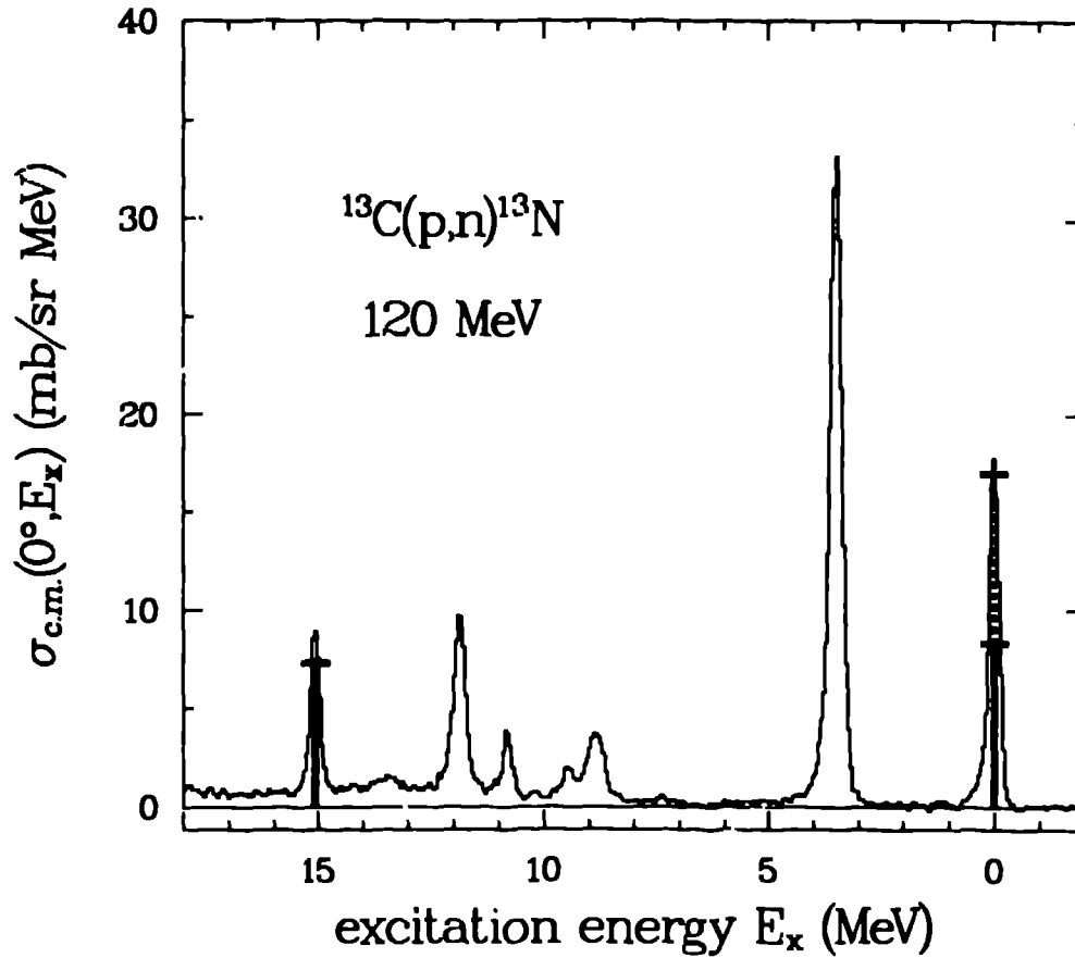
Fig. 5 Cross section spectrum for ^{13}\text{C}(p,n)^{13}\text{N} at 0^\circ and 120 MeV. The vertical bars represent the GT transition strengths for analogous beta decays. The Fermi strength is indicated by the dashed vertical line.
