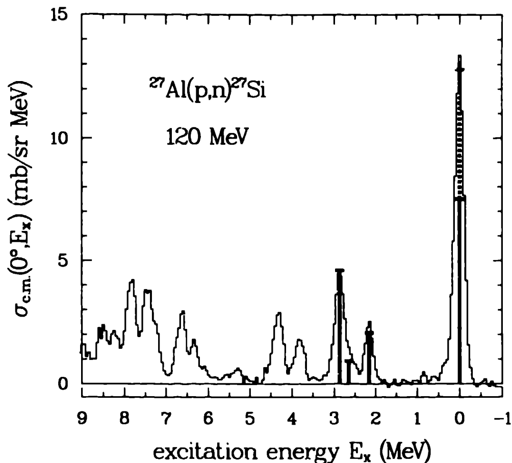
Fig. 3 Cross section spectrum for ^{27}\text{Al}(p,n) at 0^\circ and 120 MeV. The vertical bars represent the GT transition strengths for analogous beta decays. The Fermi strength is indicated by the dashed vertical line.
