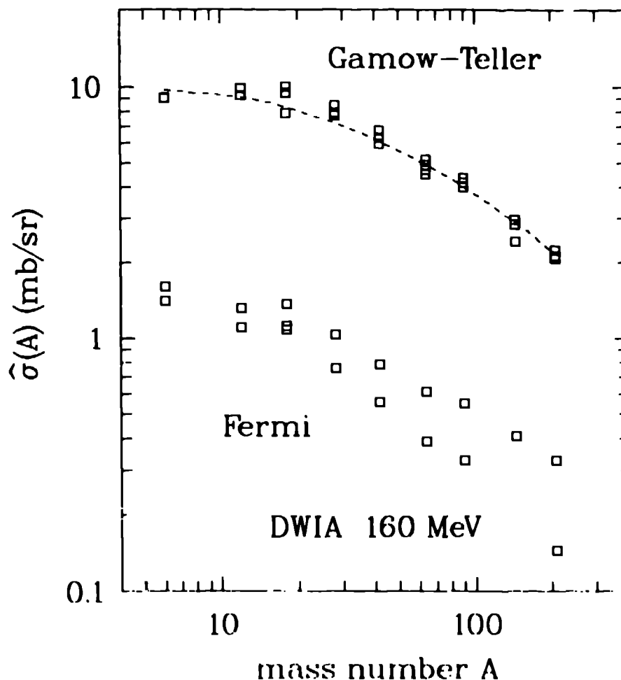
Fig. 1 Distorted-waves impulse approximation unit cross sections (squares). Multiple boxes for a given value of A correspond to different particle-hole configurations; the smallest Fermi cross sections for a given value of A correspond to |j\rangle\langle j|^{-1} transitions. The dashed line represents the average A dependence of the GT unit cross sections. (See Ref. 4).
