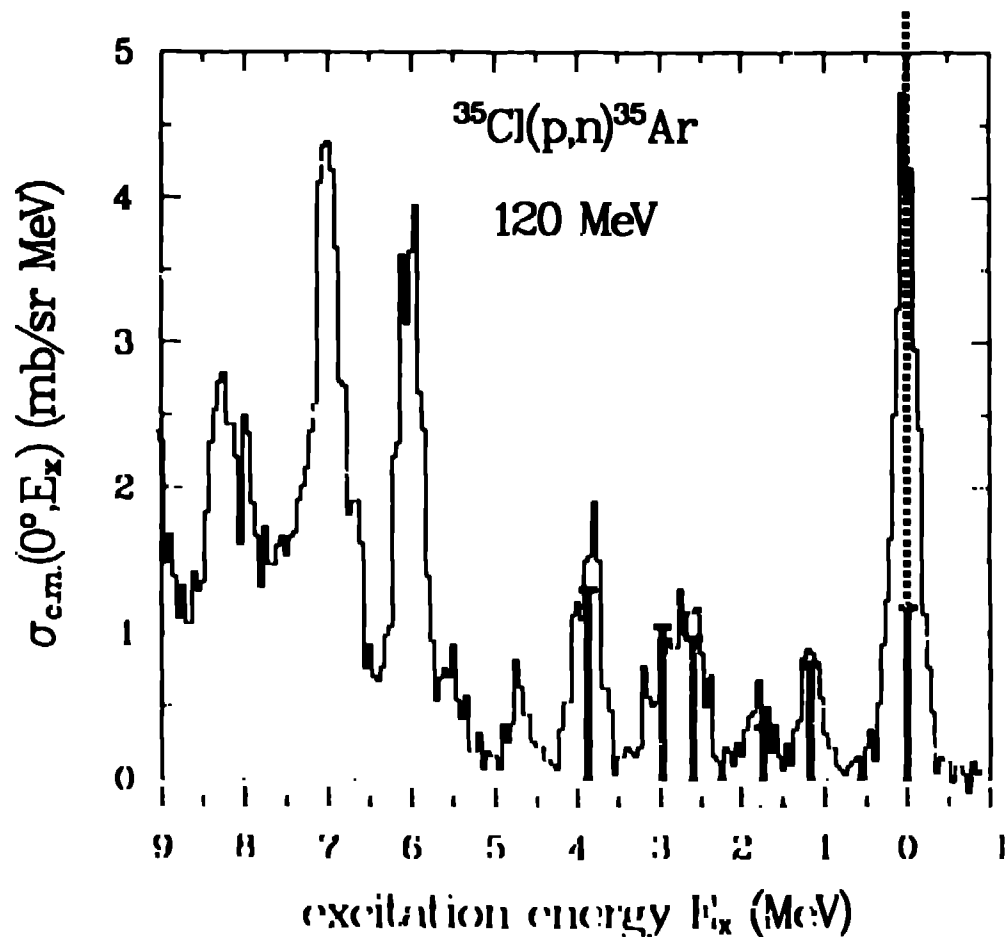
Fig. 10 Cross section spectrum for ^{35}\text{Cl}(p,n) at 0^\circ and 120 MeV. The vertical bars represent the GT transition strengths for analogous beta decays. An estimate of the Fermi cross section based on the relationship of Eq. (4) is indicated by the dashed vertical line and goes off scale.
