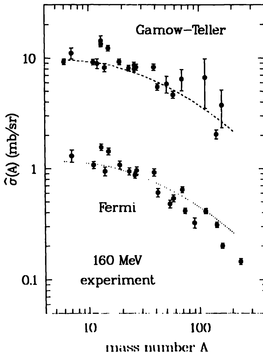
Fig. 9 Experimental unit cross sections for Gamow Teller and Fermi transitions at E_p = 160 MeV. The dashed line represents the mass dependence of the DWIA GT unit cross sections calculated with the FI. 175 MeV interaction and has not been normalized to the data. The dotted line is the dashed line divided by (160/55)^2 .
