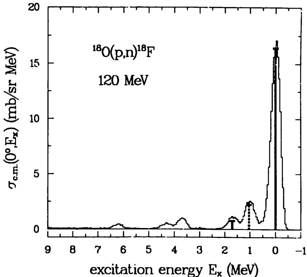
Fig. 6 Cross section spectrum for ^{18}\text{O}(p,n) at 0^\circ and 120 MeV. The solid vertical bars represent the GT transition strengths for analogous beta decays and the dashed bar represents the Fermi strength. The overall normalization for this spectrum is poorly determined.
