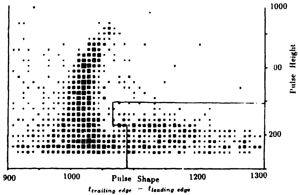
Fig. 4. Neutron separation by pulse shape.
