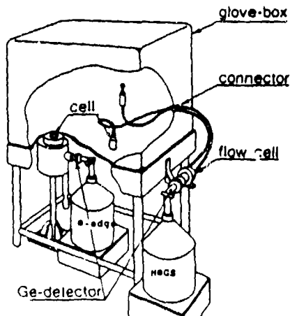
Fig. 1 Sample Cell & Detector
