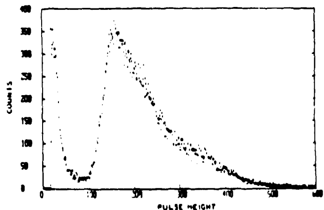
Fig. 5. Pulse height distribution for one of the ^{235}\text{U} fission chamber deposits.
