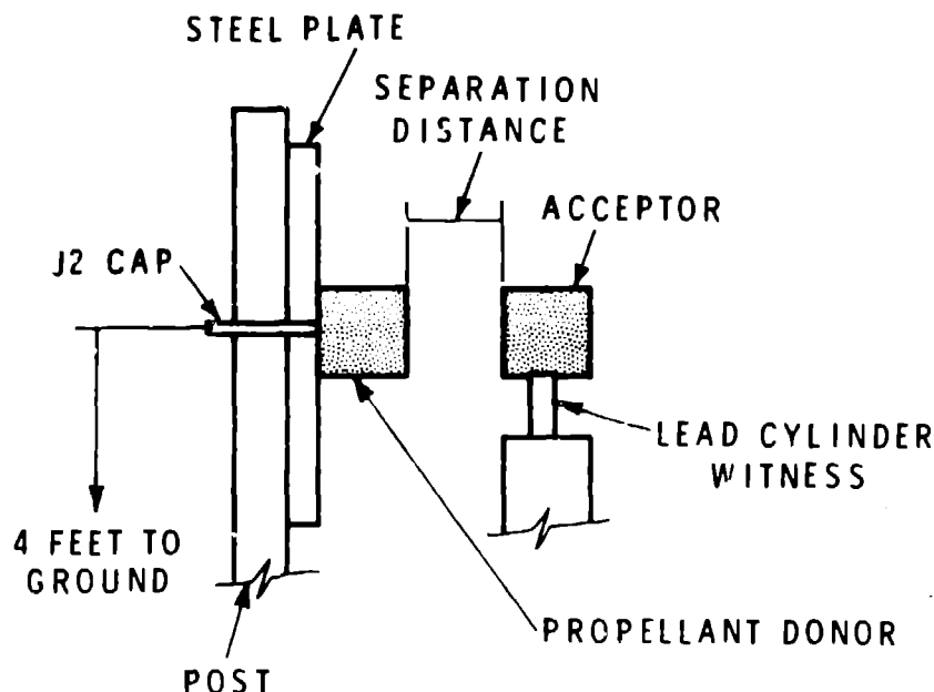
Fig. 1. Test setup for sympathetic detonation experiment.
