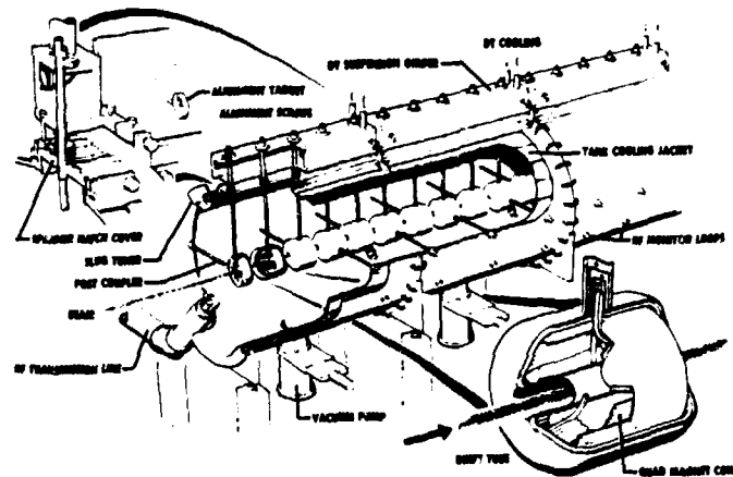
Fig. 7. Conceptual design of the drift-tube Linac tank and drift-tube support system.
