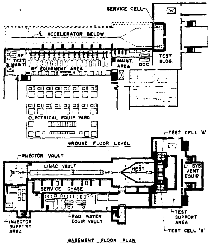
Fig. 2. FMIT Facility layout from Title I Design Studv.
