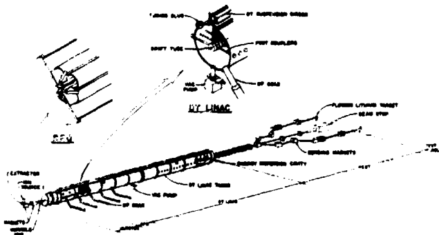
Fig. 3. Pictorial schematic of FMIT Linac components.
