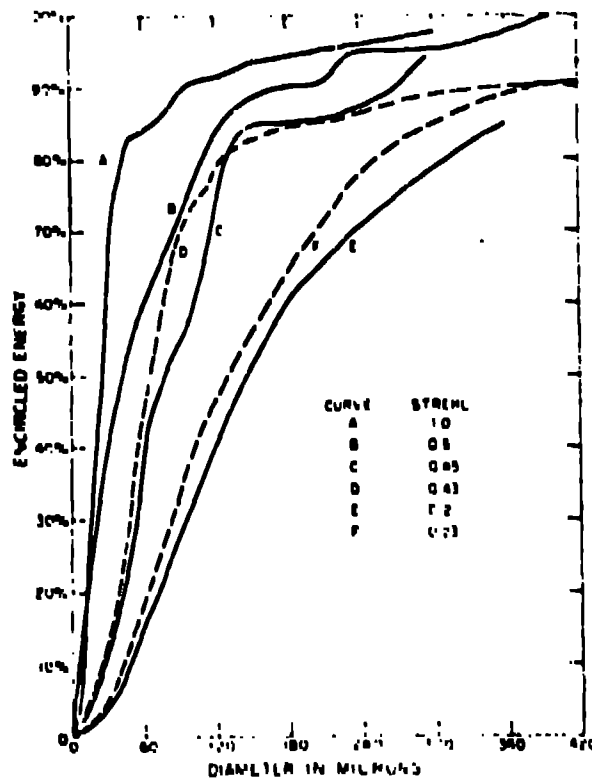
Fig. 5. Encircled and captured energy values for various Strehls.
