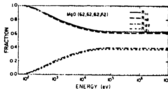
Figure 1. Values of the ratio R_{ijk} for the material MgO (62,62,62,62) as a function of PKA energy.
