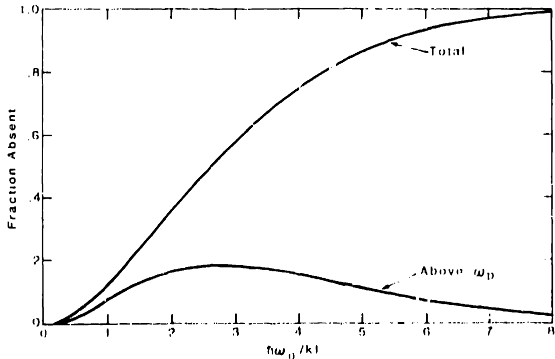
FIGURE 2 Fraction of Vacuum Blackbody Radiation Absent in a Plasma
