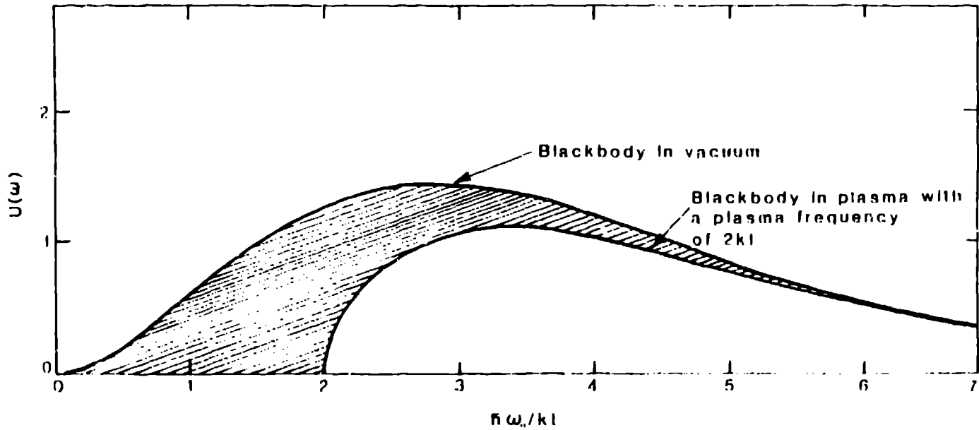
FIGURE 1 Equilibrium Radiation Energy Density
