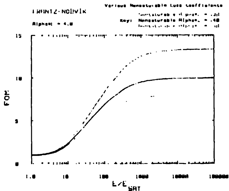
Figure 2. Model calculations for a Finite Noise Absorber with a nonsaturable loss and \alpha = 4 . A nonsaturable loss of 0.35 represents the practical case of Mix 907.
