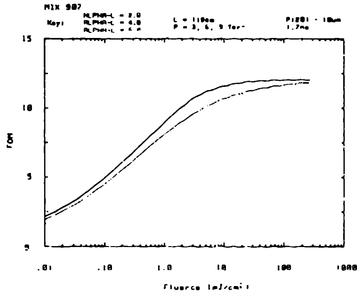
Figure 3. The measured FOM of gas Mix 907 for small-signal loss lengths of 2, 4, and 6 at P(20) = 10 \text{ m} with 1.7 ns pulses of Gaussian space time radiation. Maximum FOM is 12.
